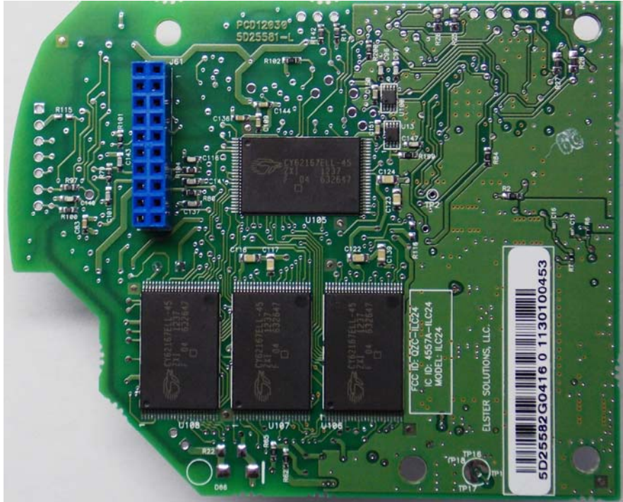
Figure 1 – 900 MHz ILC2 PCBA (BOTTOM)
