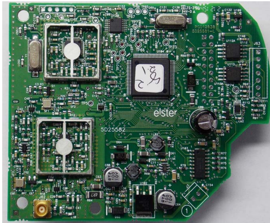
Figure 2 – 900 MHz ILC2 PCBA (TOP)
