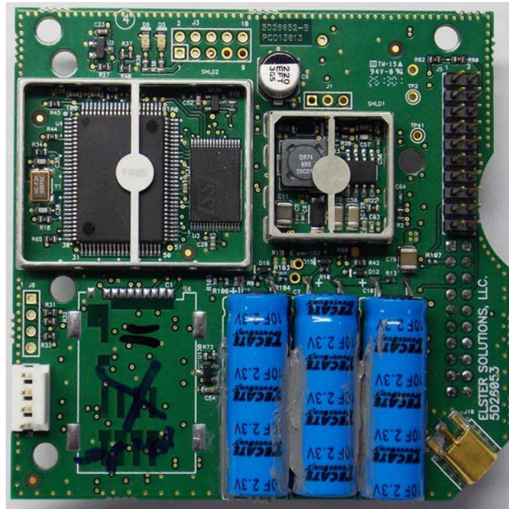
Figure 4 - WWIC3G EV-DO PCBA (TOP)
