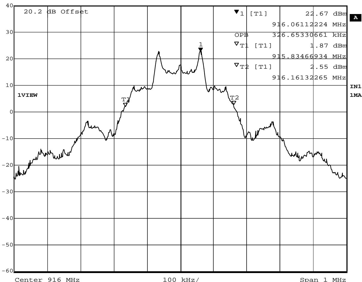
Figure 9 – 99% Power Bandwidth = 326.7 kHz
