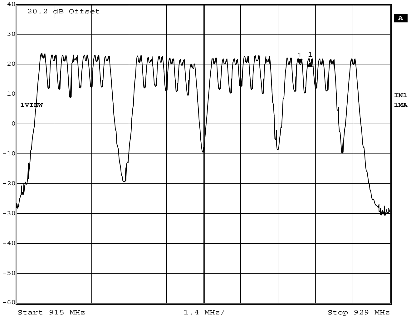
Figure 5: Plot of hopping Channels 915-928 MHz (Upper Band)
