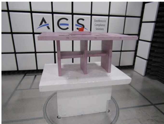
Figure 2: Radiated Emissions – Front View – Above 1GHz – 451 MHz Radio
