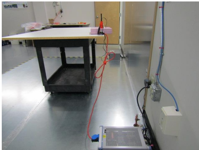
Figure 6: Powerline Conducted Emissions – Side View – 900 MHz Radio
