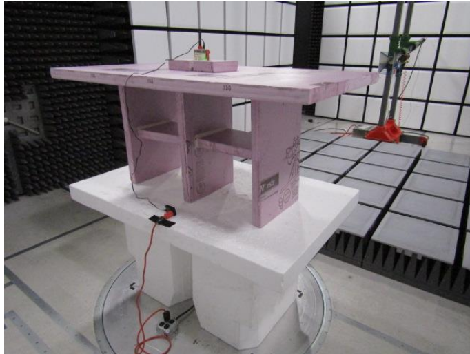
Figure 4: Radiated Emissions – Back View – Above 1GHz – 900 MHz Radio
