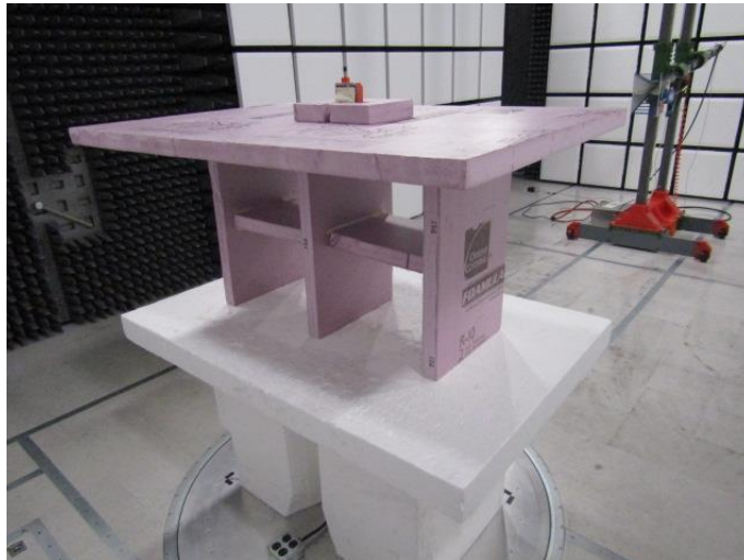
Figure 1: Radiated Emissions – Back View – Above 1GHz – 451 MHz Radio
