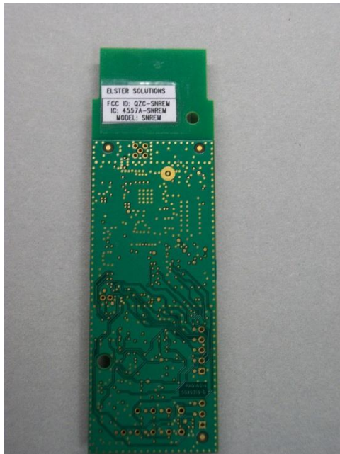
PCB Back:
