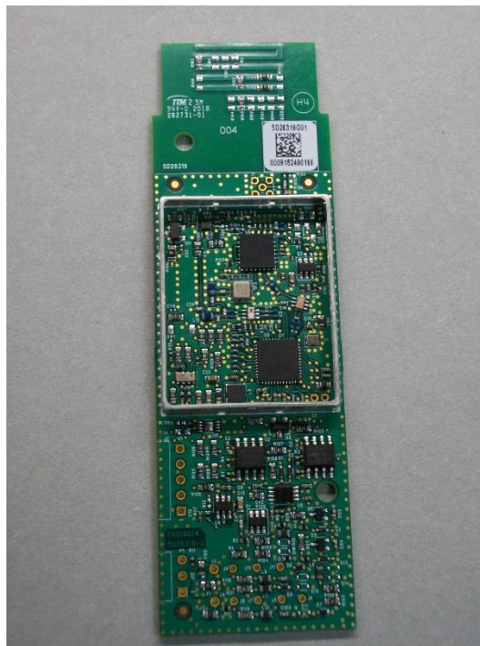
PCB Front with Shield Lid Removed:
