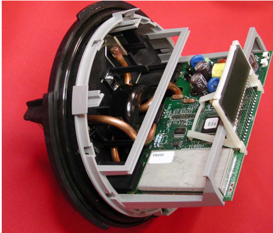
Figure1: REX Meter without Outer Cover and Inner Housing Removed
