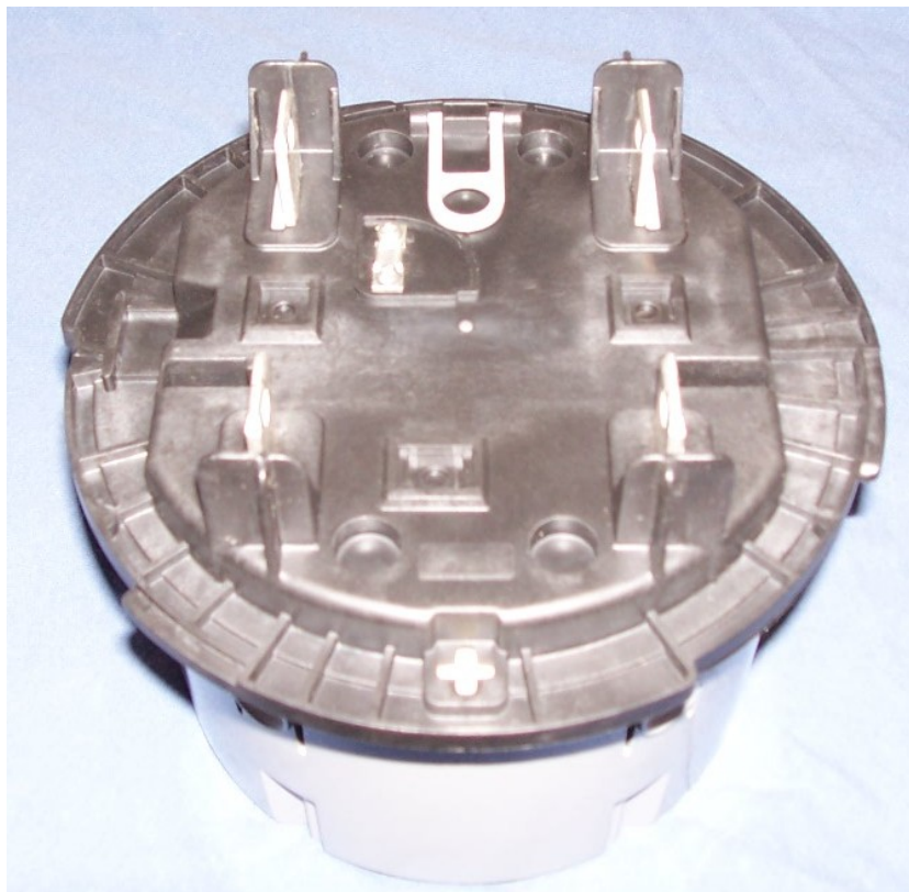
Figure 4: Bottom View
