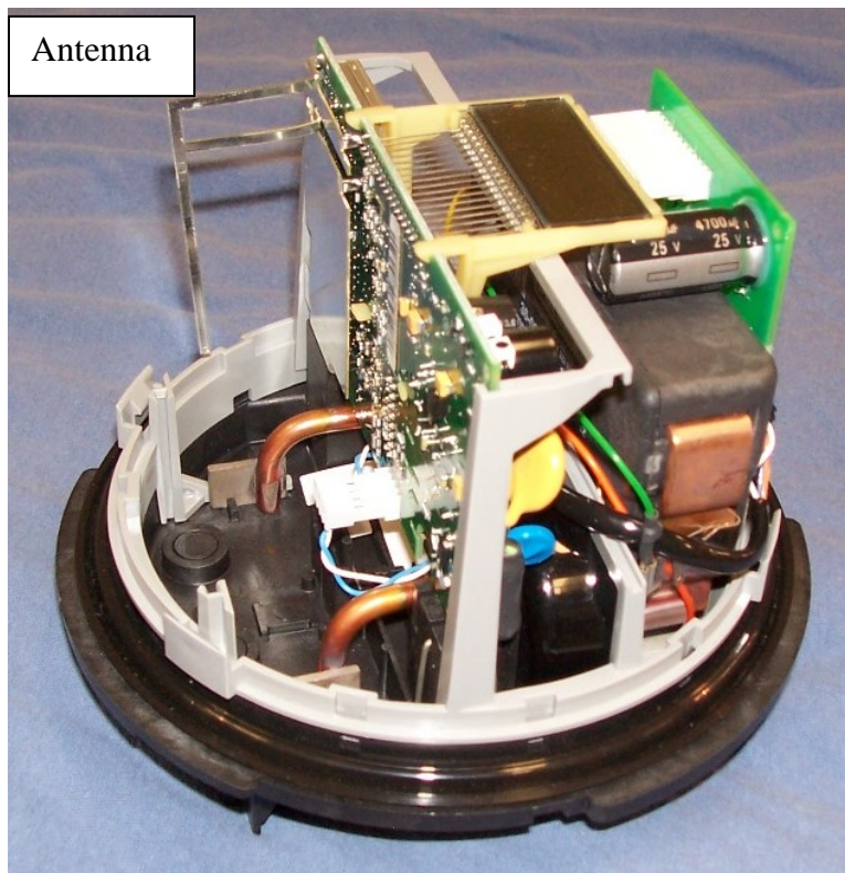
Figure 2: REX Meter with internal service disconnect switch
