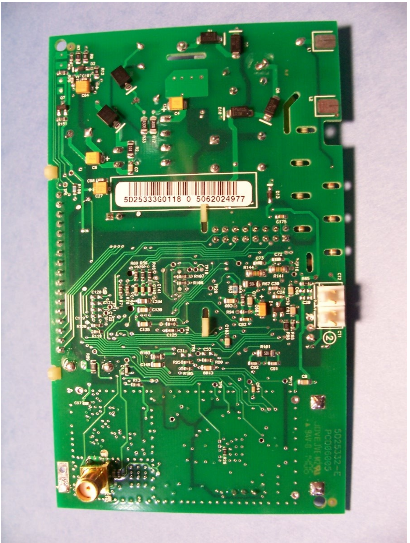
Figure 5: Bottom View of Transceiver Board
