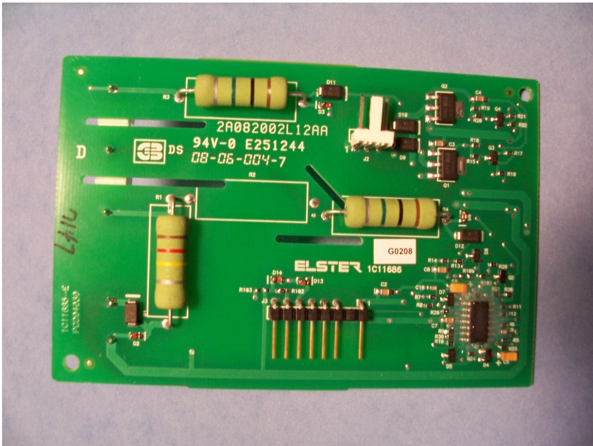
Figure 7: Top View of Disconnect Board
