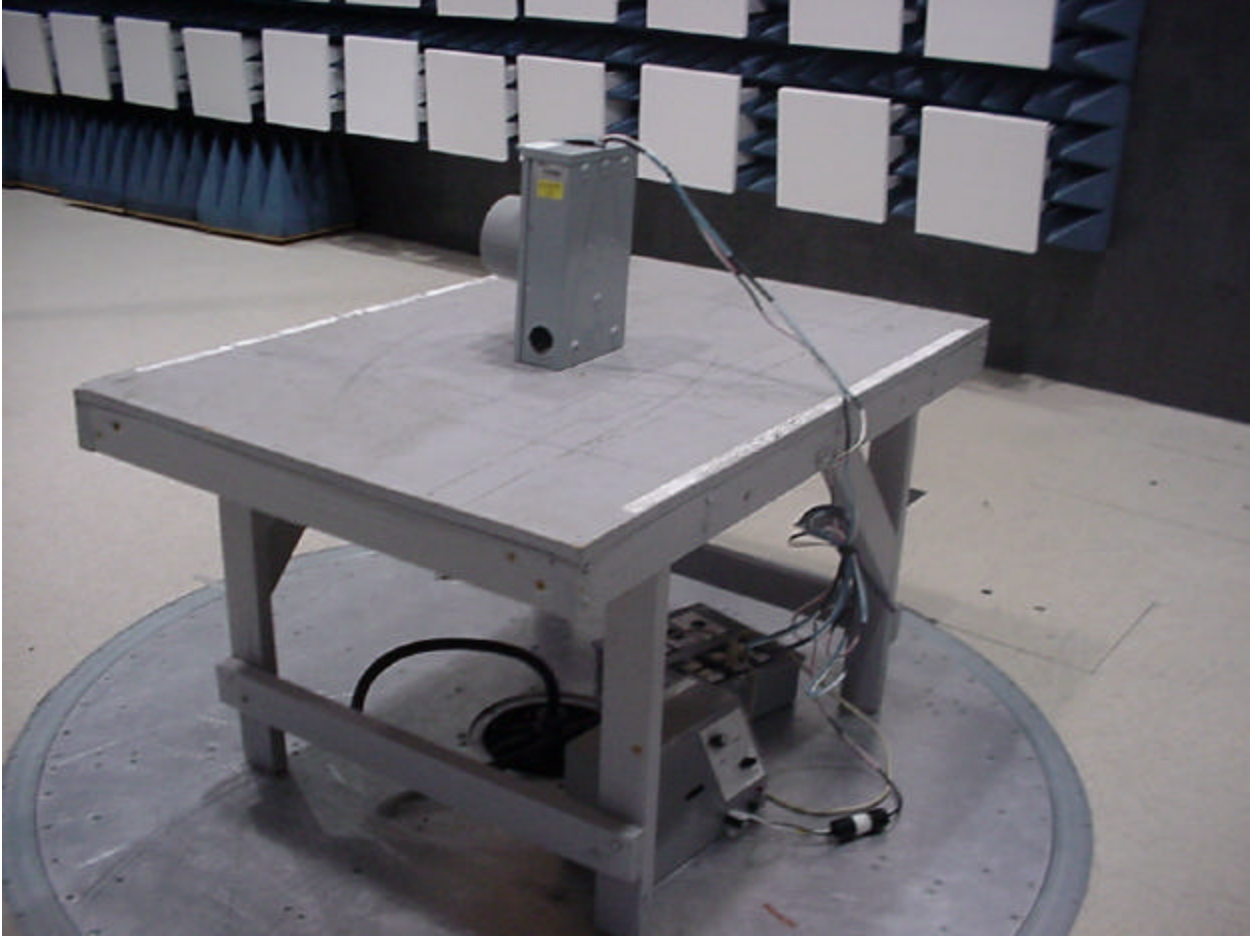
Figure 2 - Radiated Emissions Test Setup (Chamber - Back)
