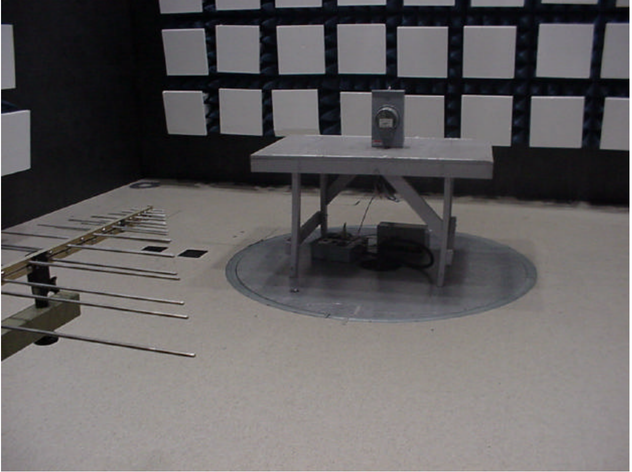
Figure 1 - Radiated Emissions Test Setup (Chamber - Front)
