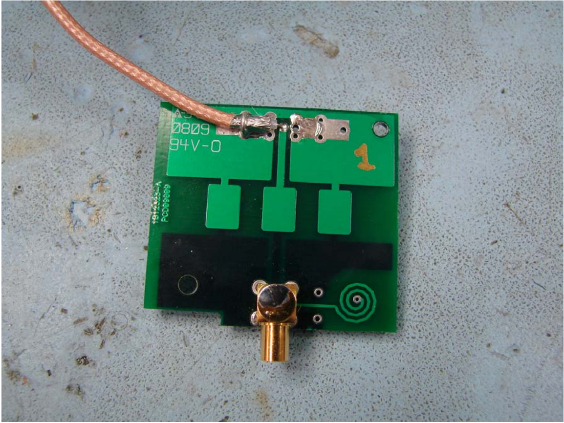
Top View Antenna Isolation Board
