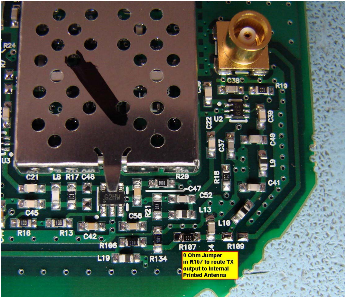
Jumper Position for Internal Antenna
