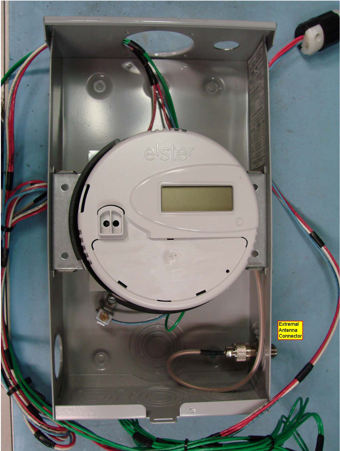
Installation of Meter in Socket Box with External Antenna Connection
