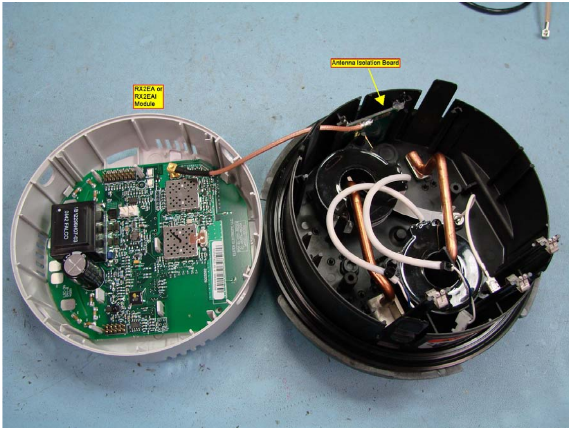
Connection of Antenna Isolation Board
