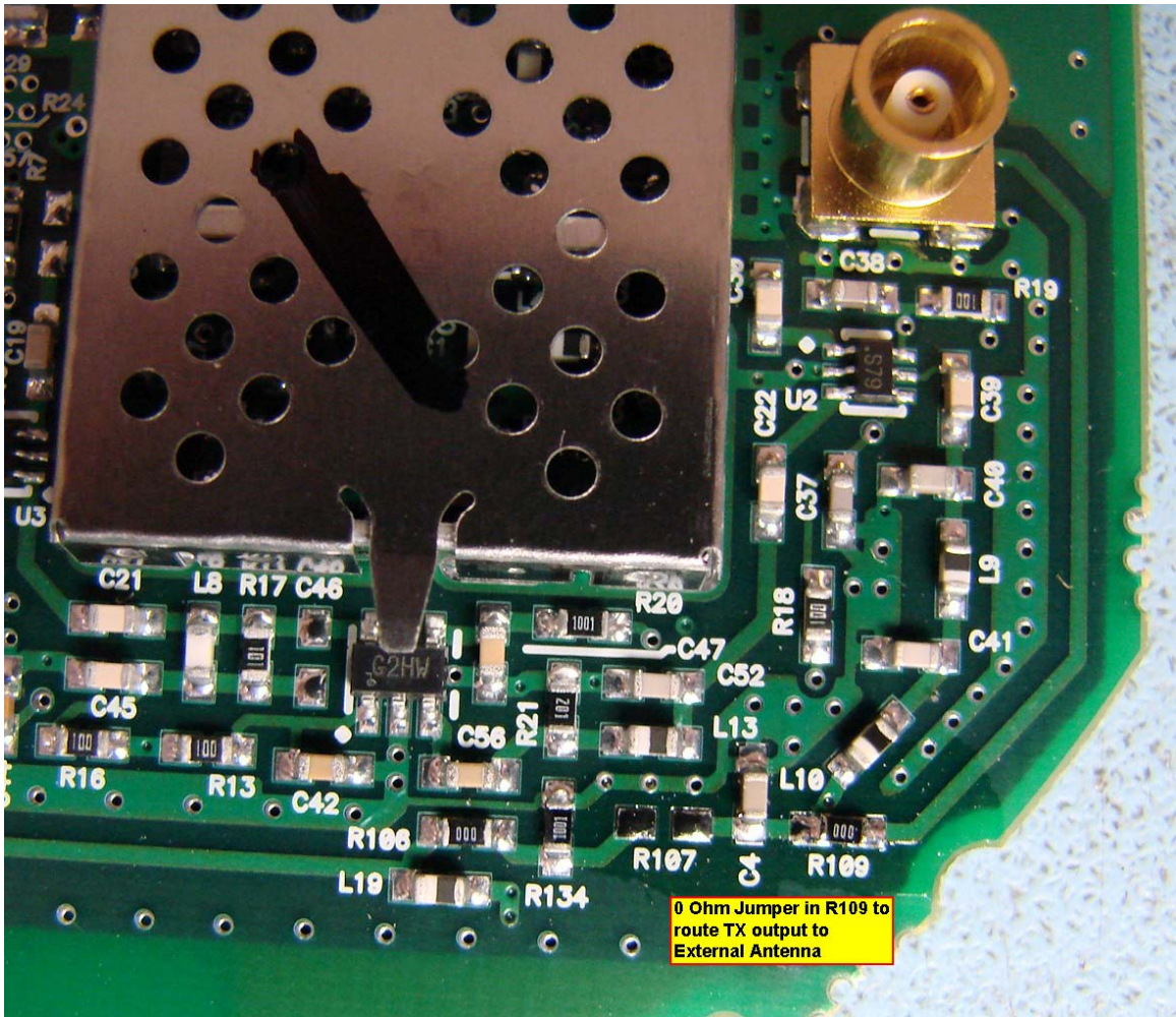
Jumper Position for External Antenna
