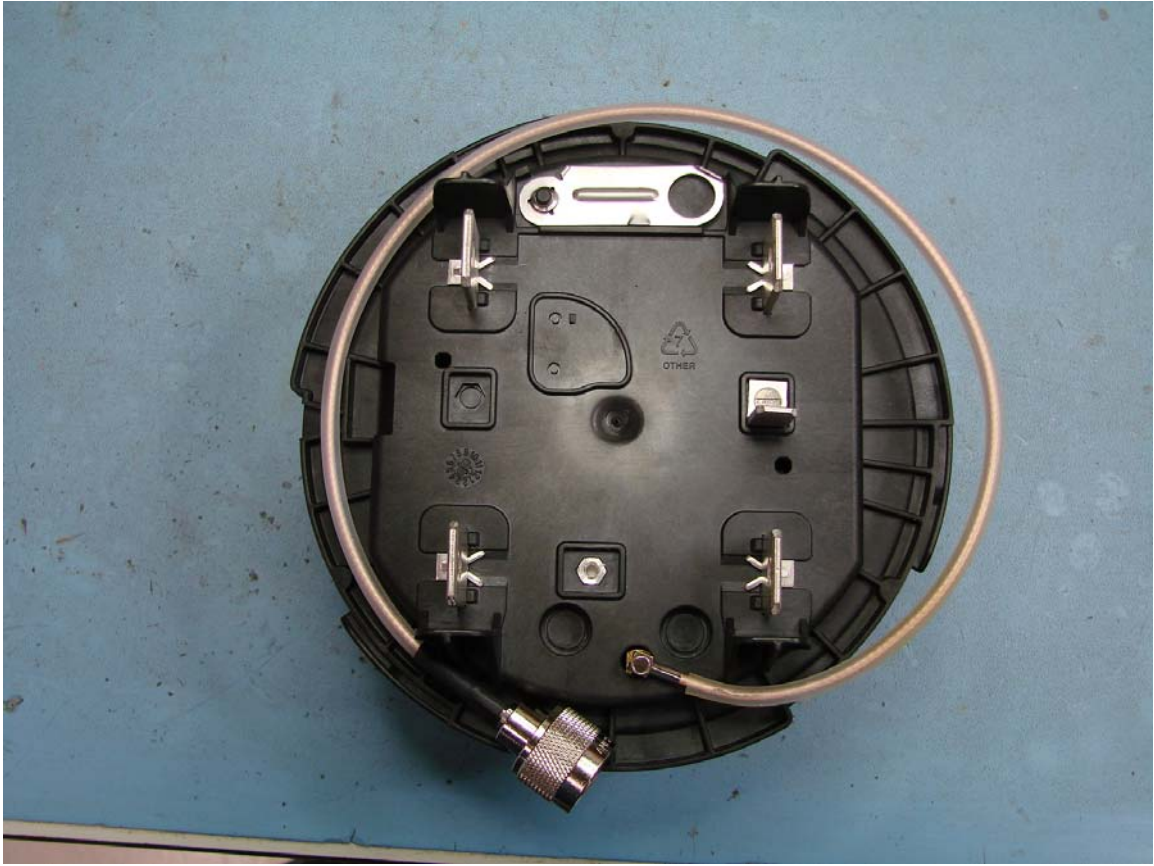
Bottom View of Meter Base with Cable for External Antenna
