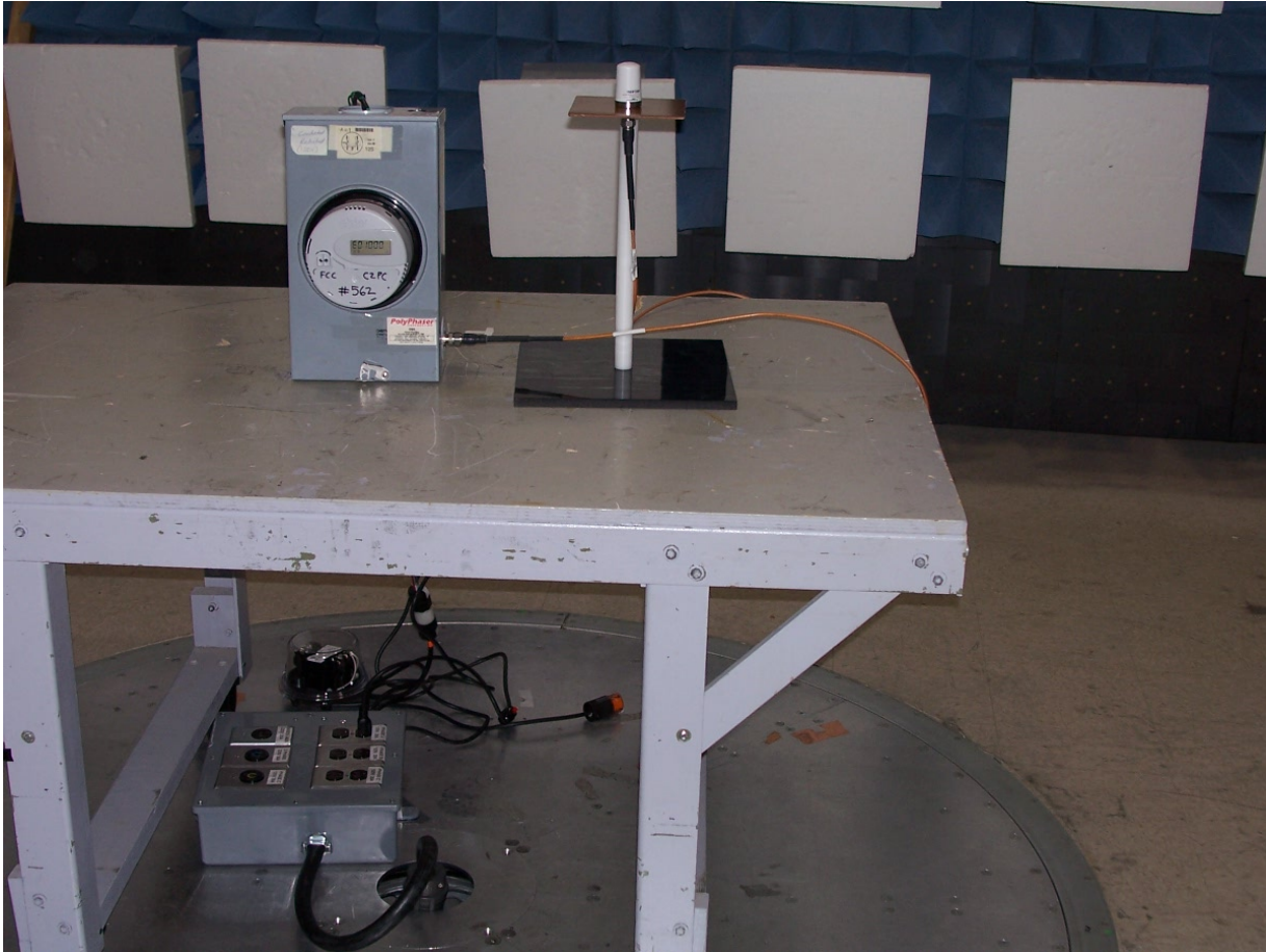
Front View of Test Setup with the Antenex TRAB9023NP Antenna
