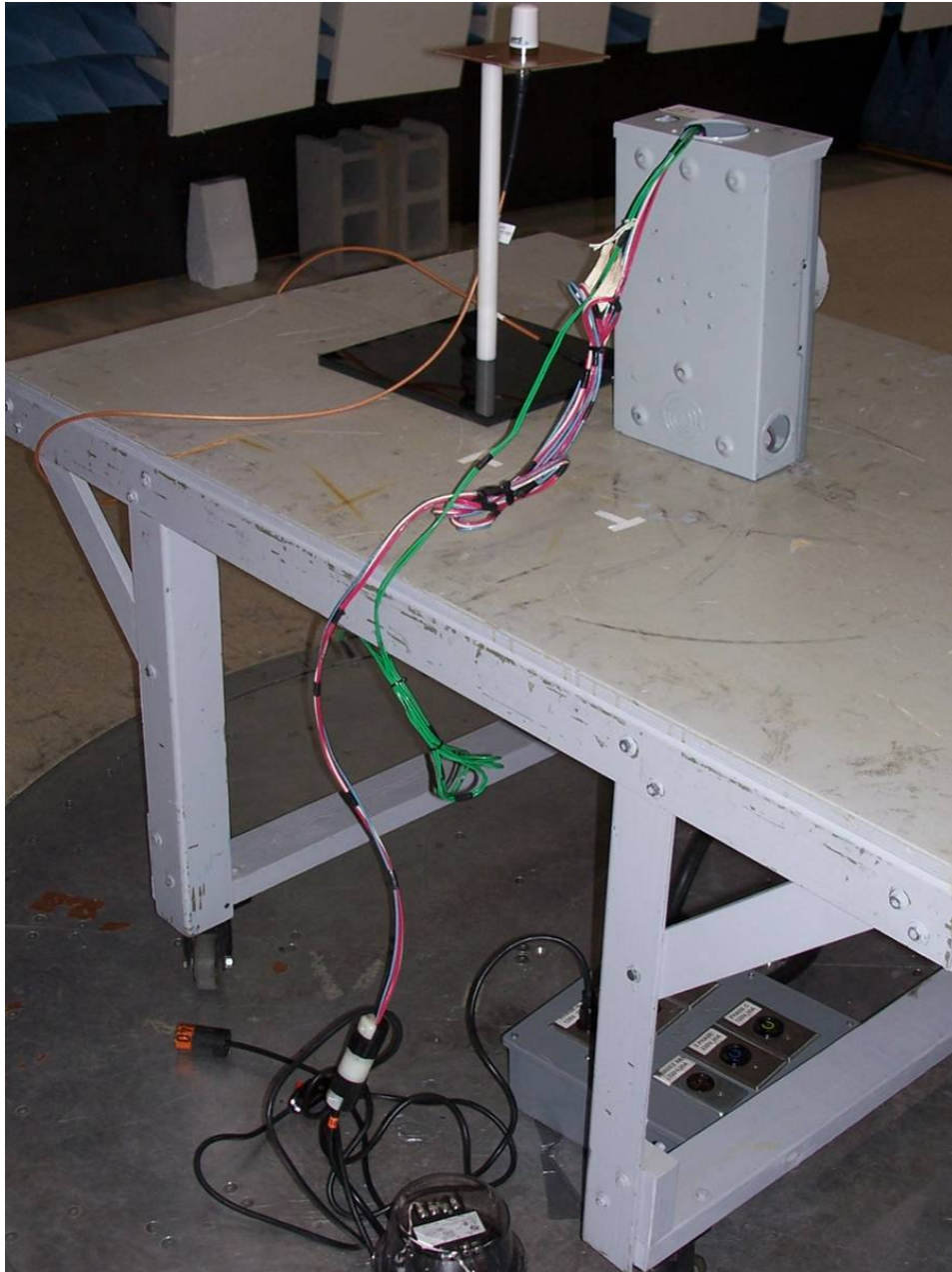
Rear View of Test Setup with the Antenex TRAB9023NP Antenna
