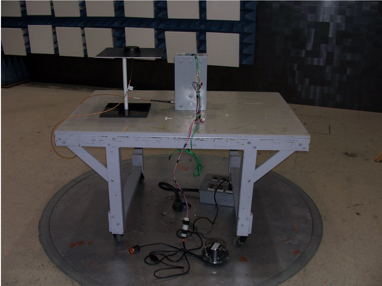
Rear View of Test Setup with the Larsen LP800NMO Antenna
