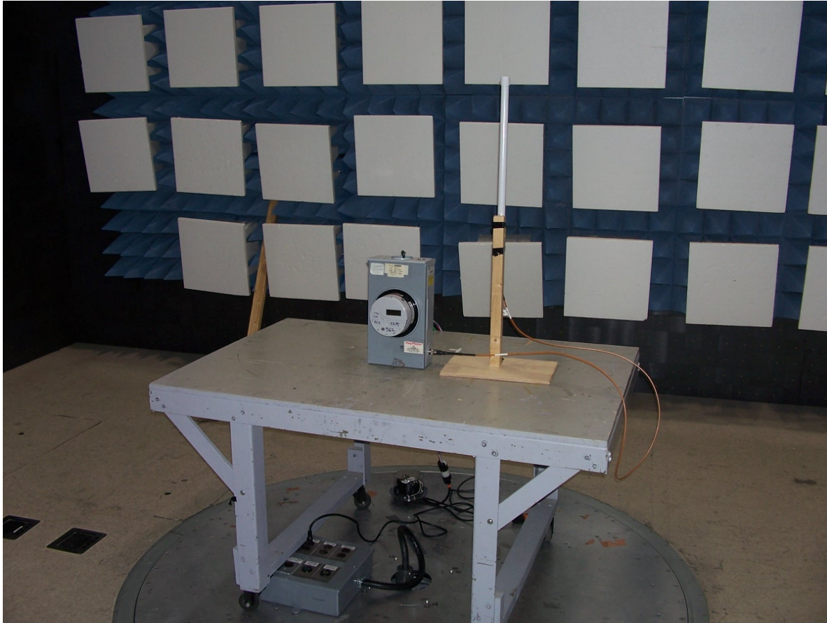
Front View of Test Setup with the PCTEL (MAXRAD) MFB9150 Antenna
