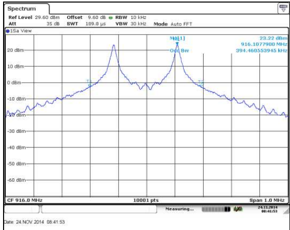
Figure 7.4.4.2-4: 99% BW Low Channel
