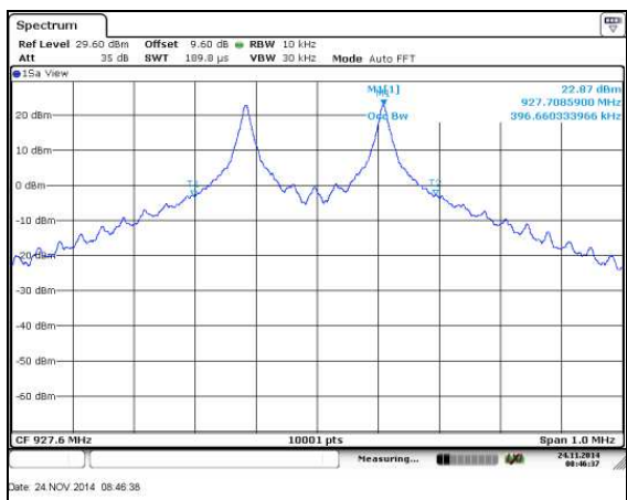
Figure 7.4.4.2-6: 99% BW High Channel
