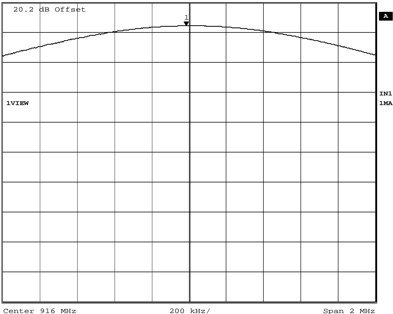
Figure 11: CH 34 (916.0 MHz) Peak Output Power
