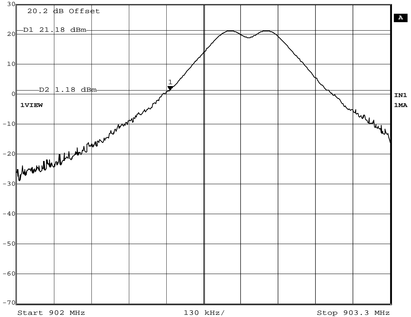
Figure 1: Lower Band Edge Measurement
