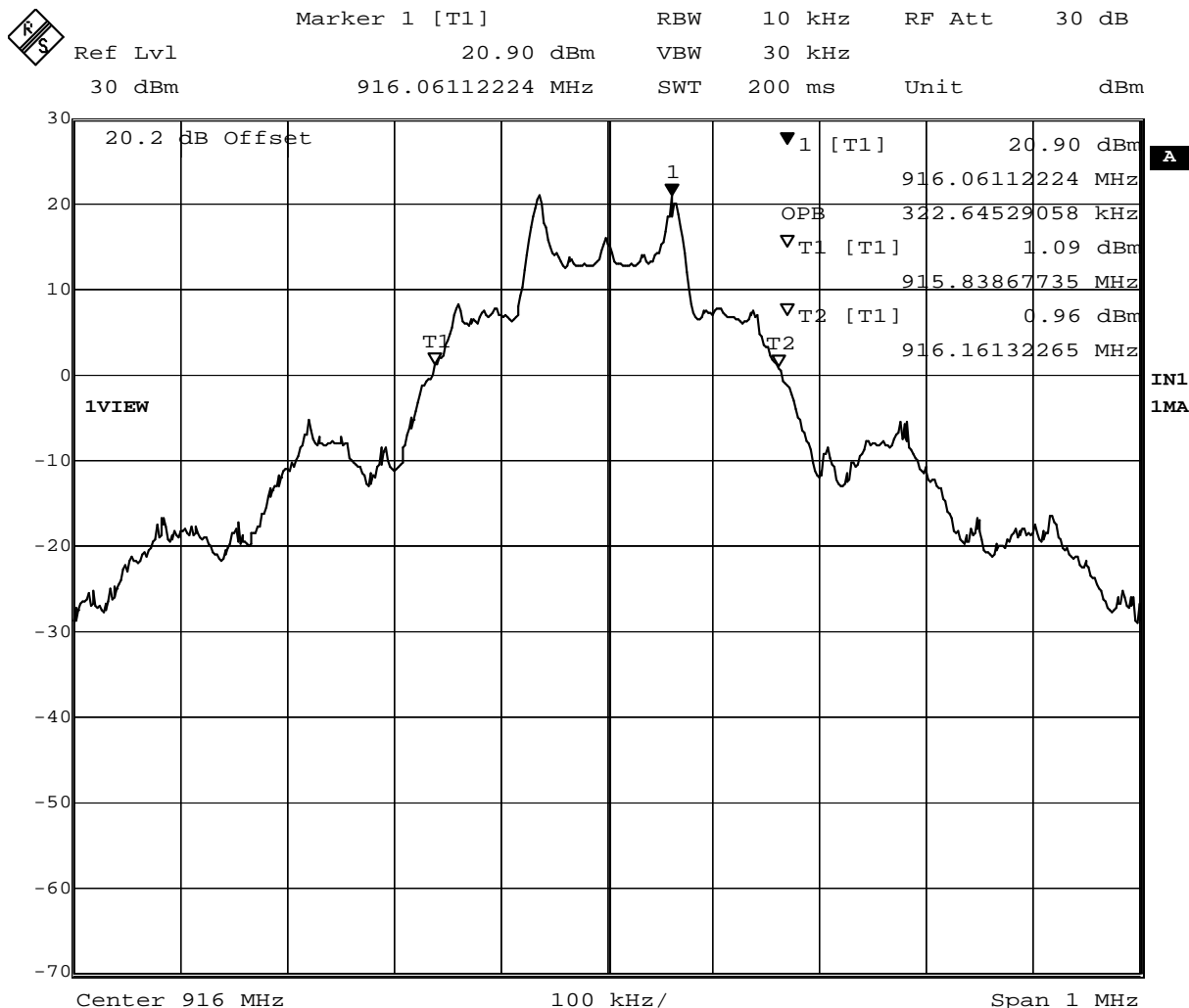
Figure 9 – 99% Power Bandwidth = 322.6 kHz
