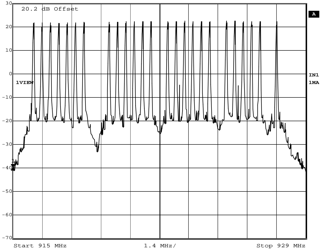
Figure 5: Plot of hopping Channels - 915-928 MHz (Upper Band)
