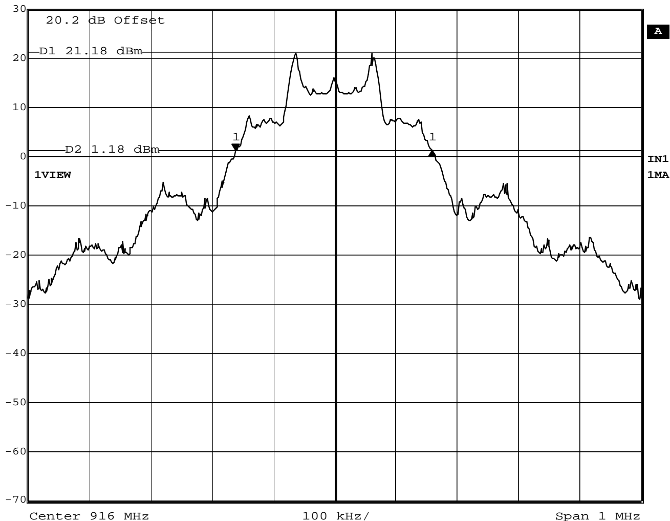
Figure 8: Occupied Bandwidth
