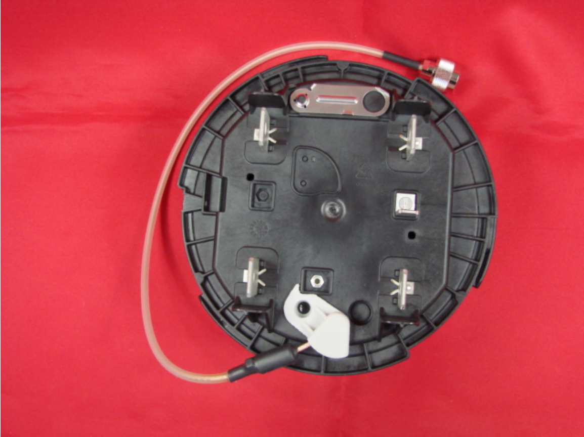
Figure 7: Rear View
