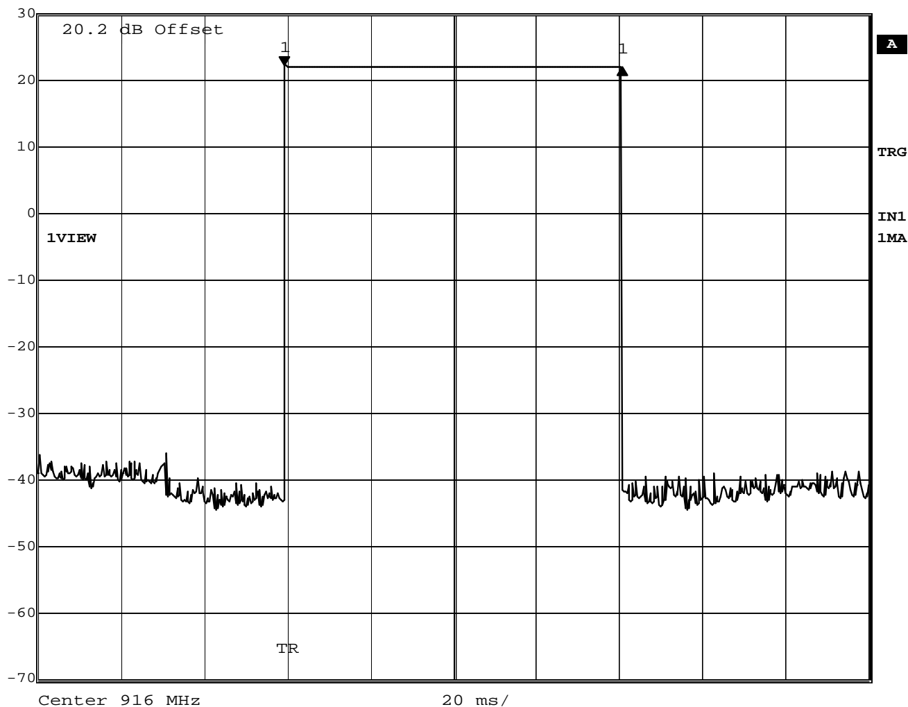
Figure 6: Measurement of 1 hop at 916.0 MHz
