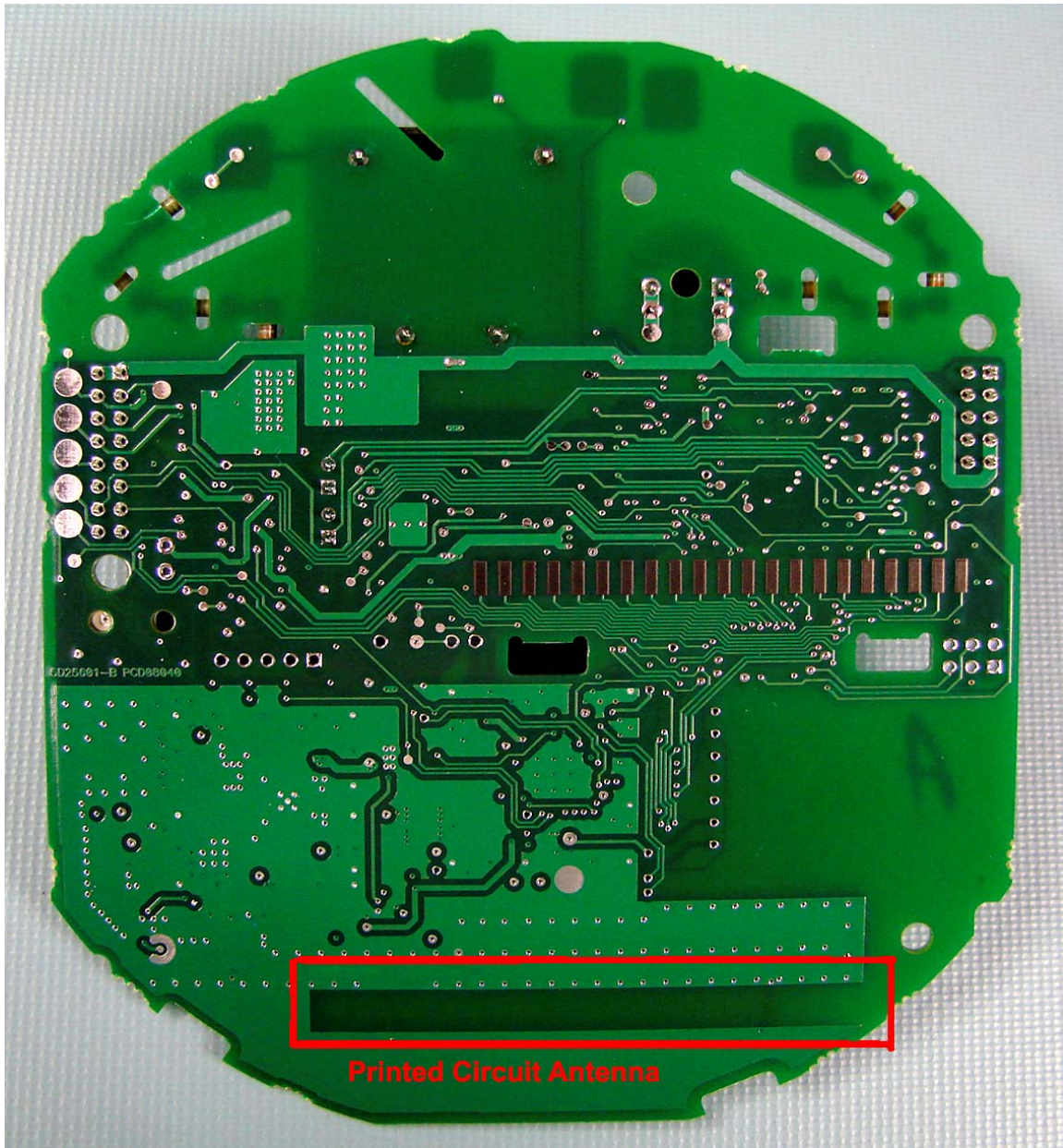
INTERNAL PRINTED CIRCUIT BOARD SHOWING PRINTED CIRCUIT ANTENNA
