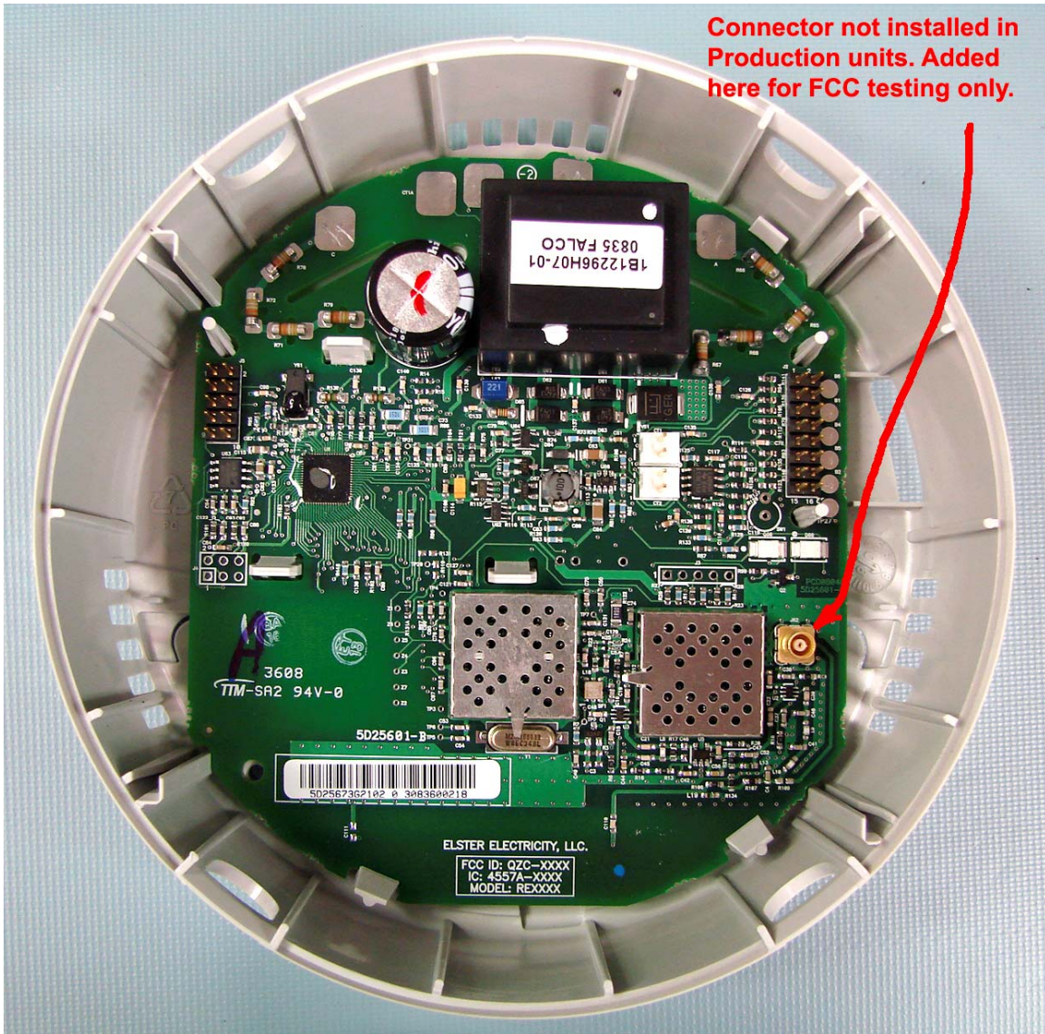
INTERNAL ASSEMBLY SHOWING PCBA INSTALLED IN HOUSING
