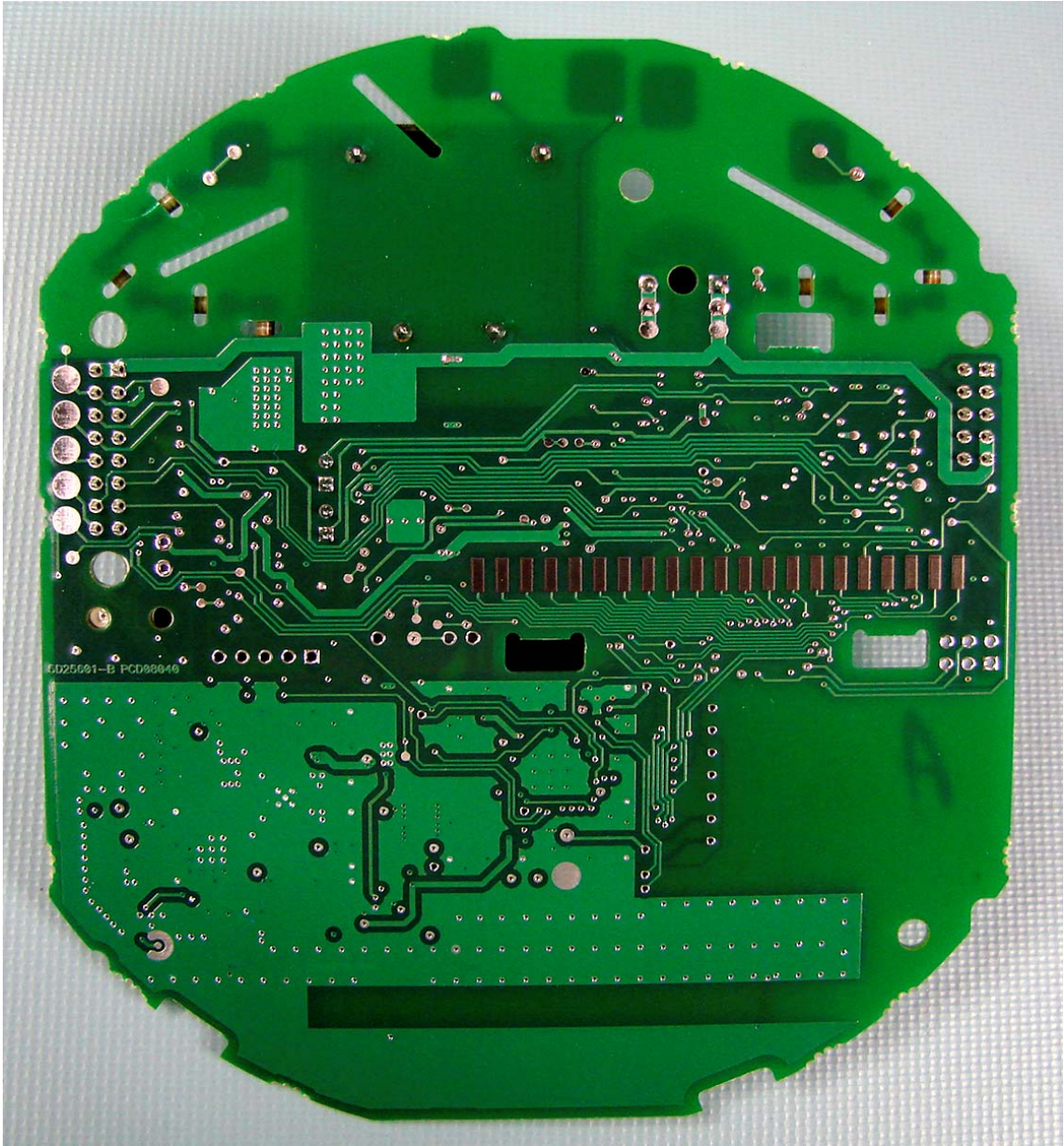
INTERNAL PRINTED CIRCUIT BOARD ASSEMBLY BOTTOM VIEW
