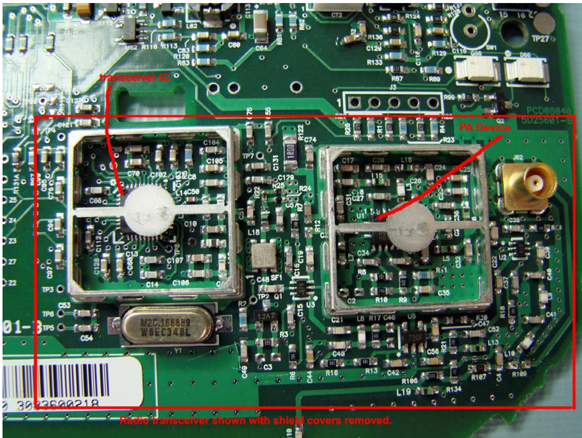
INTERNAL PRINTED CIRCUIT BOARD SHOWING 915 MHZ RADIO WITH SHIELD COVERS REMOVED
