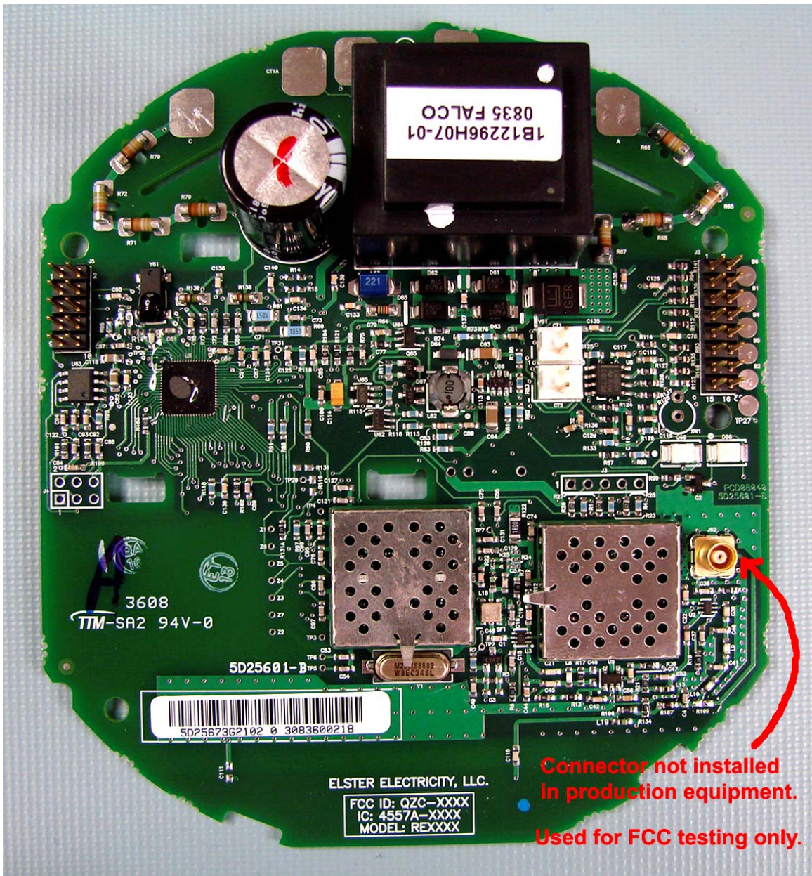
INTERNAL PRINTED CIRCUIT BOARD ASSEMBLY TOP VIEW
