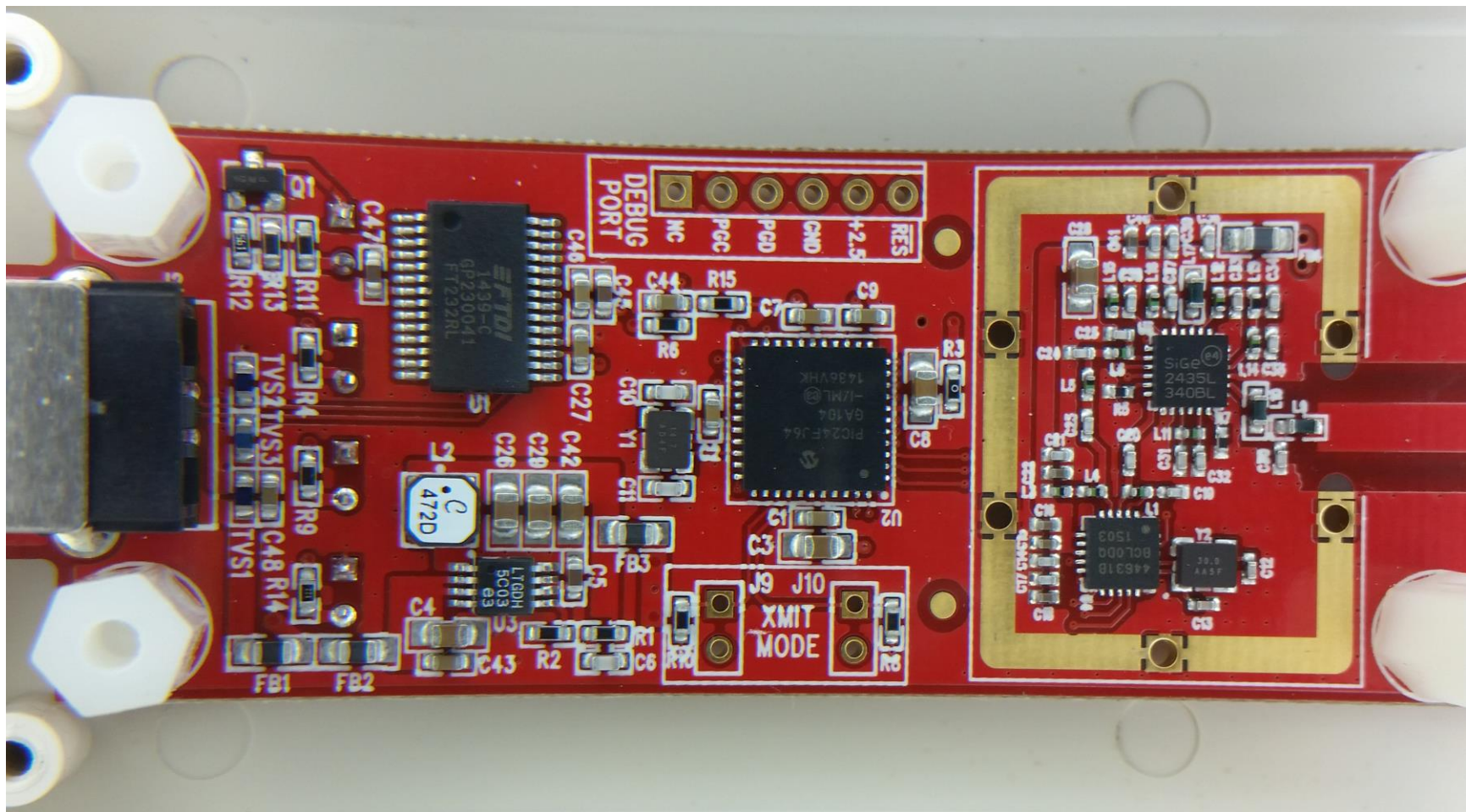
Figure 4. Close-up of the board with metal shield removed.
