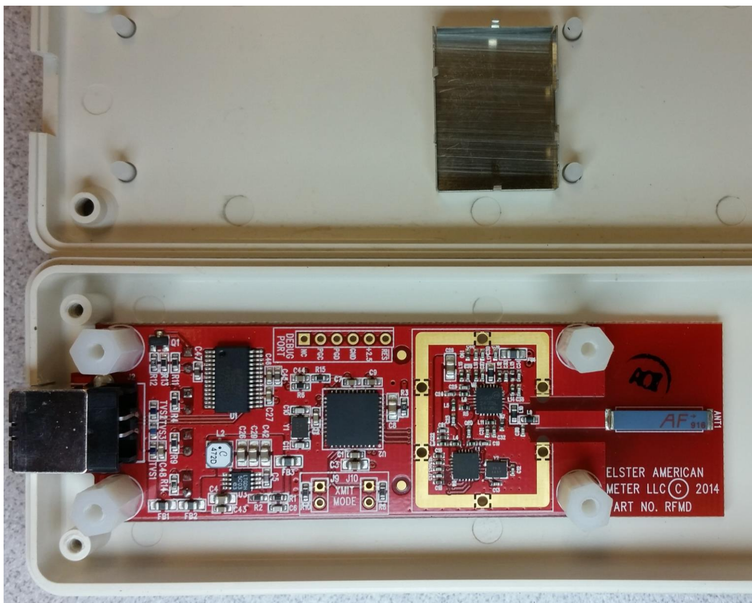
Figure 3. Metal shield removed.
