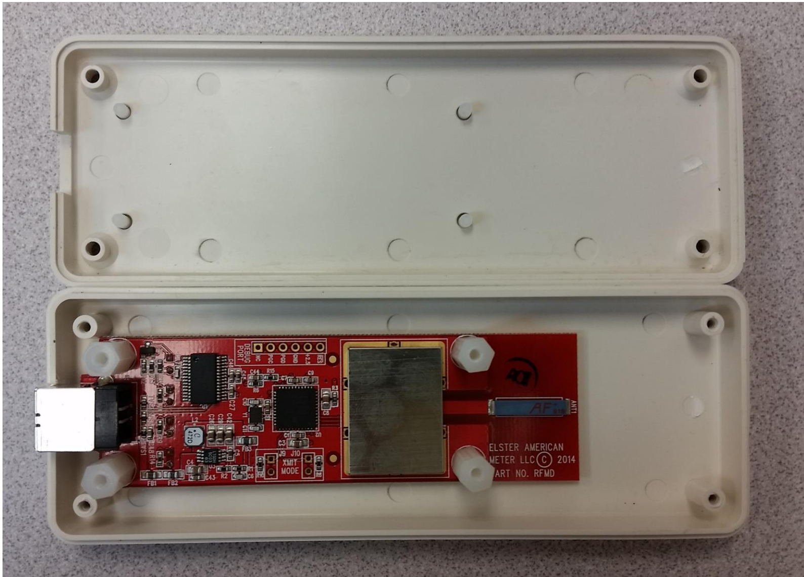
Figure 2. Board is turned over.
