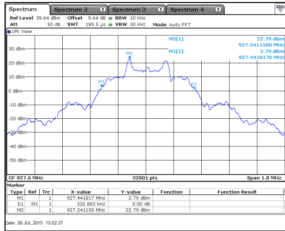
Figure 7.4.4.2-12: 20dB BW High Channel – 142.2kpbs
