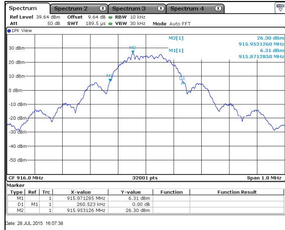
Figure 7.4.4.2-10: 20dB BW Mid Channel – 200kpbs
