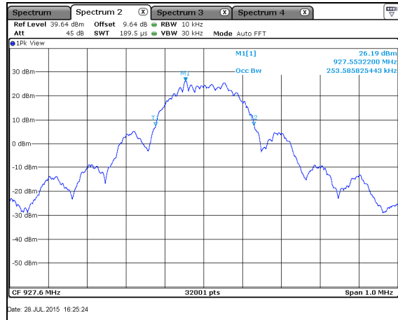
Figure 7.4.4.2-30: 99% BW High Channel – 200kbps
