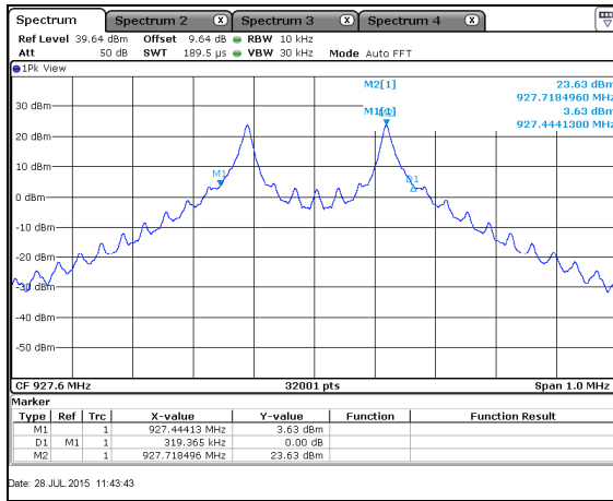
Figure 7.4.4.2-11: 20dB BW High Channel – 35.5kpbs
