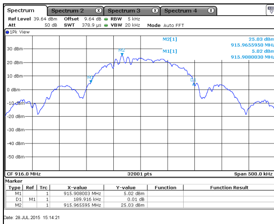
Figure 7.4.4.2-9: 20dB BW Mid Channel – 150kpbs
