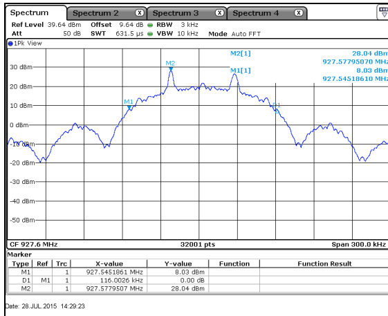
Figure 7.4.4.2-13: 20dB BW High Channel – 50kpbs
