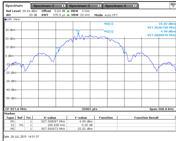
Figure 7.4.4.2-14: 20dB BW High Channel – 150kpbs
