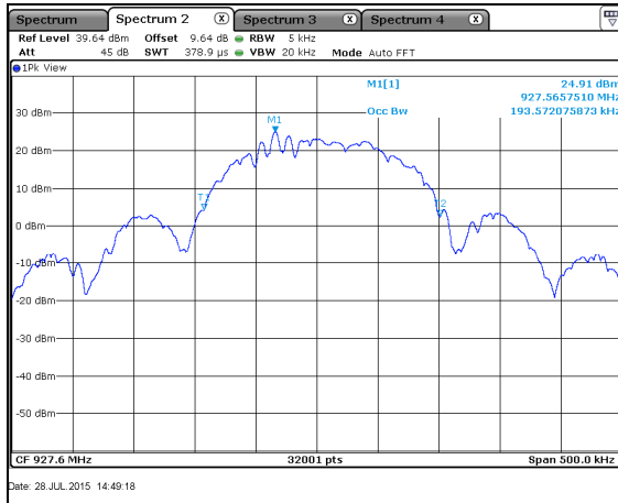
Figure 7.4.4.2-29: 99% BW High Channel – 150kbps
