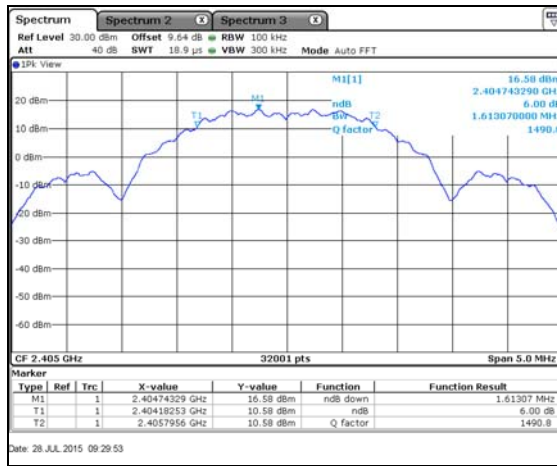
Figure 7.3.2-1: 6dB Bandwidth Plot – LCH
