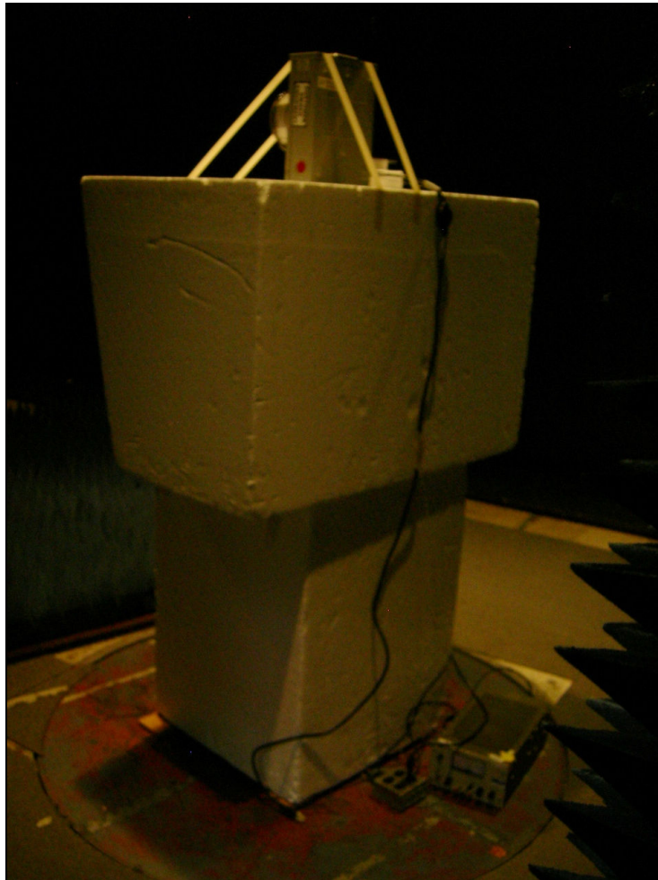
Figure 3: Radiated Emissions
