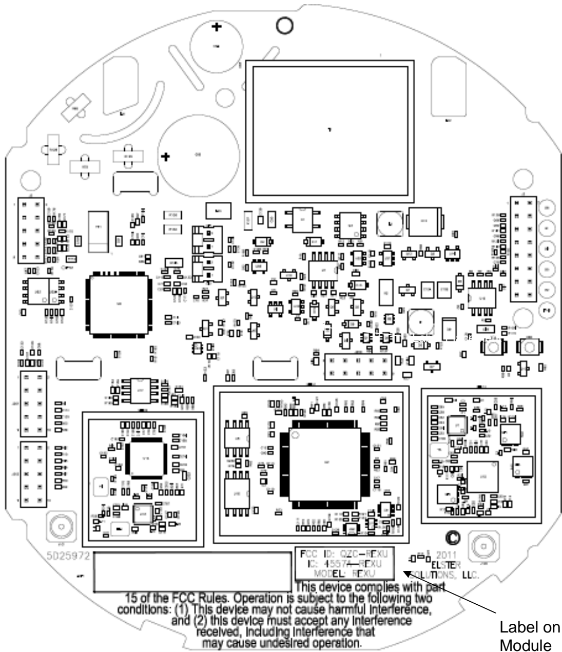
Figure 2: Label Placement
