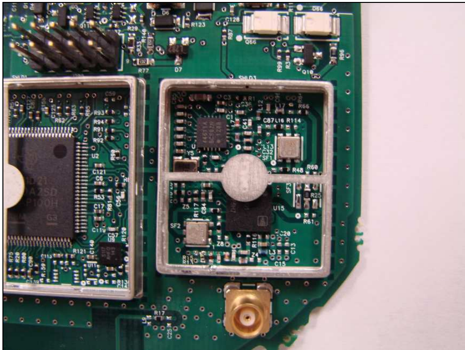
Figure 3: Internal Photo Close-up – Shields Removed
