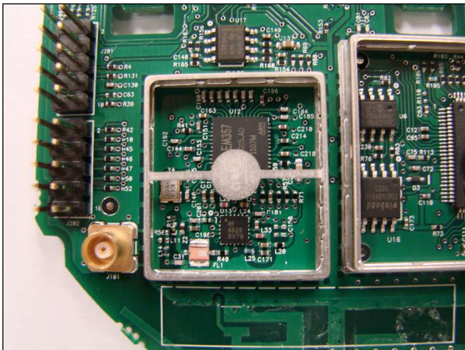
Figure 2: Internal Photo Close-up – Shields Removed
