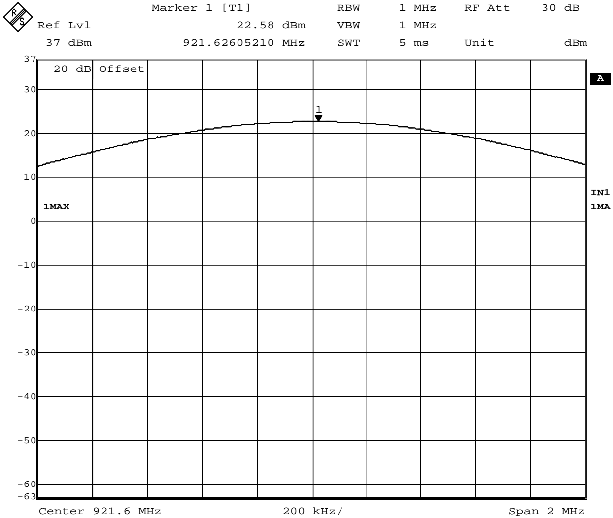
Figure 6: CH 48 (921.626 MHz) Peak Output Power
