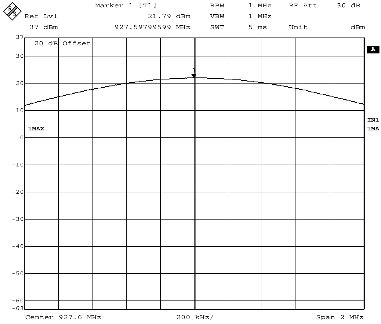
Figure 7: CH 63 (927.597 MHz) Peak Output Power
