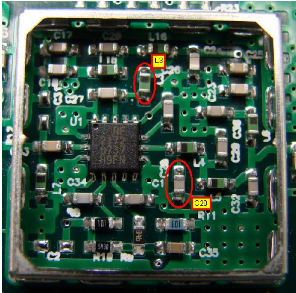
Changes made to R2EAI Power Amplifier Shield Cover Removed
