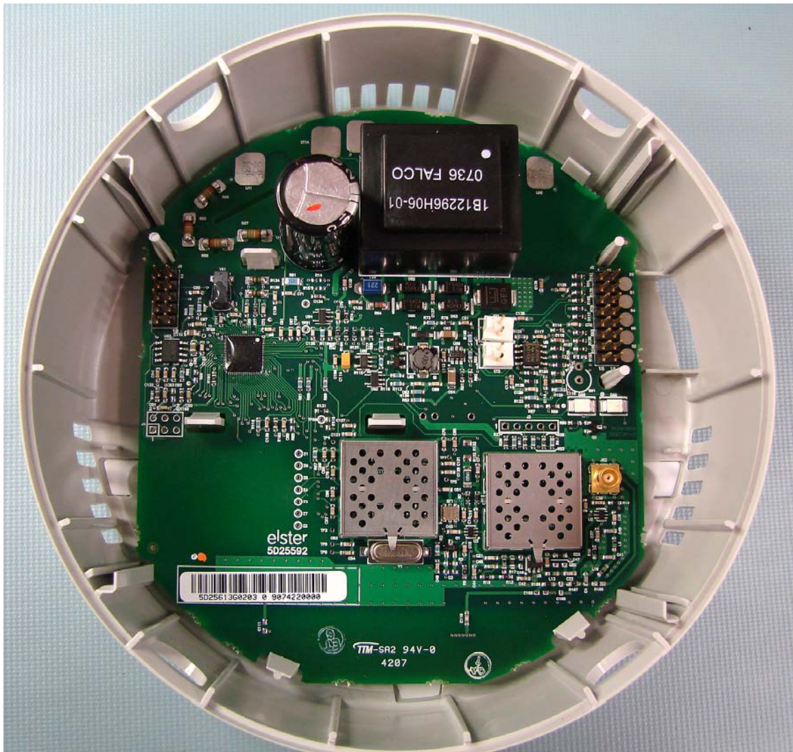
INTERNAL ASSEMBLY SHOWING PCB INSTALLED IN FRONT COVER
