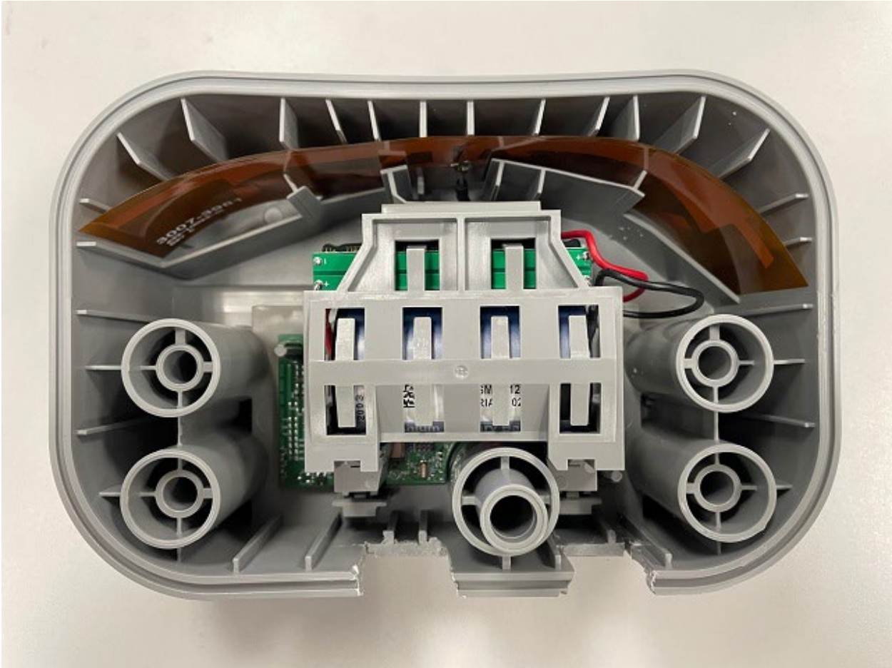
Housing interior, rev B shown, rev E is the same
