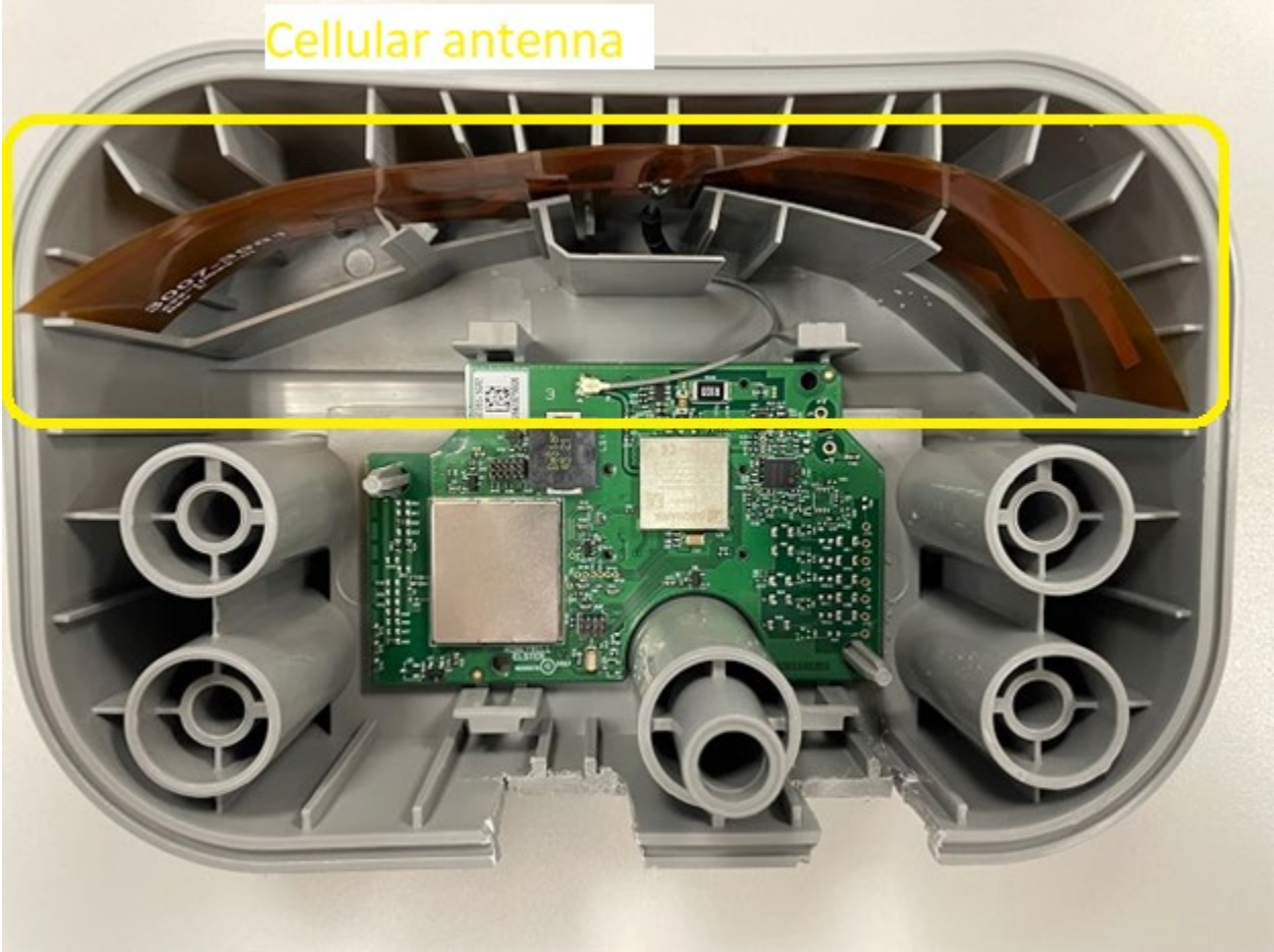
Housing interior showing PCB and antennae (battery omitted for clarity), rev B shown, rev E is the same
