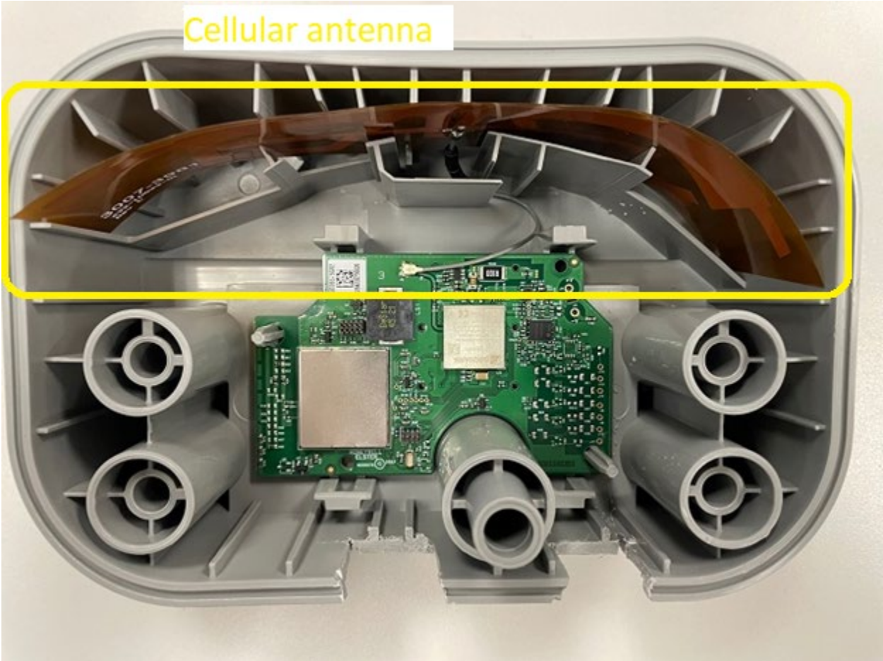
Housing interior showing PCB and antennae (battery omitted for clarity)
