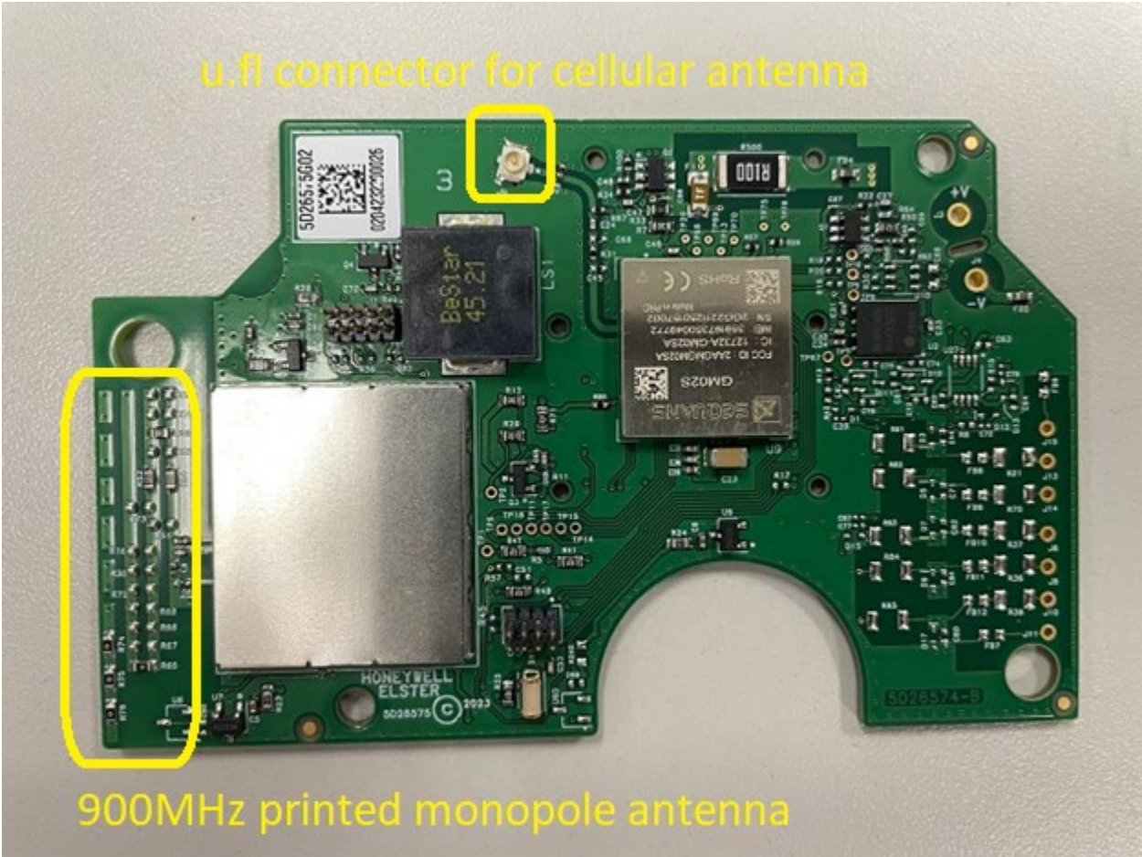
PCB top side with shield can lid installed
