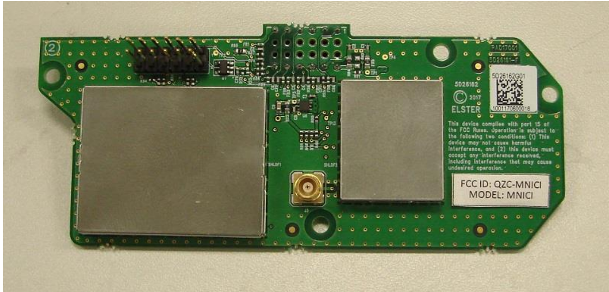
SynergyNet Mini Network Interface Card (MNIC) Printed Circuit Board Assembly (PCBA) top view
