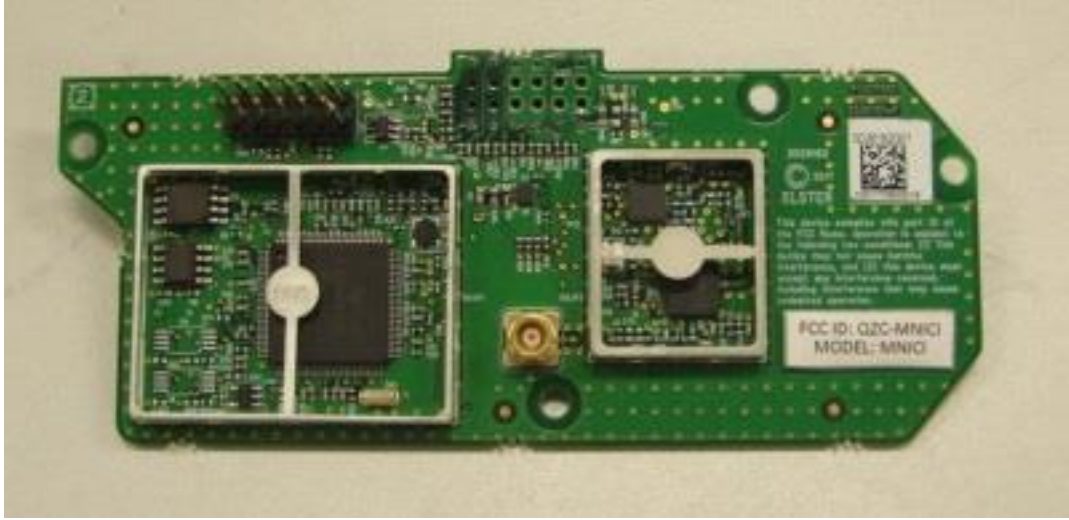
MN1C1 PCBA top view, shield can lids removed
