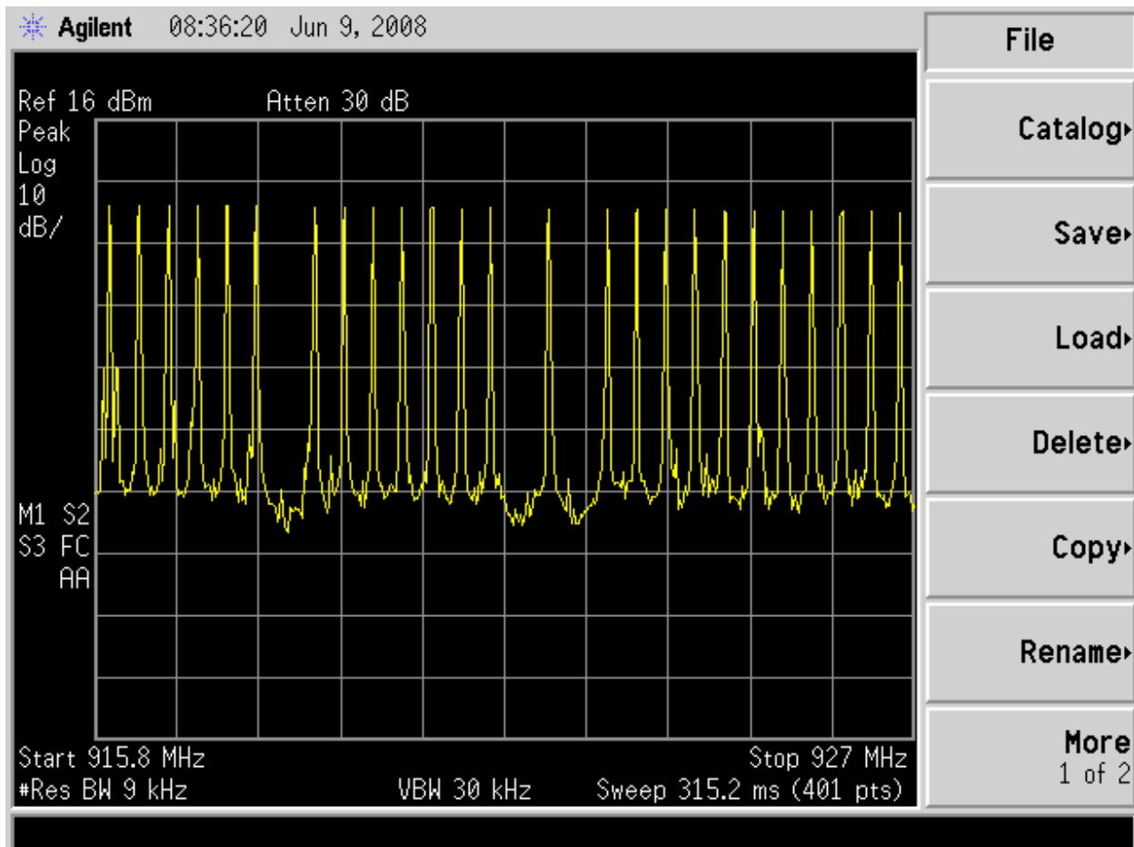
Figure 2 - Plot of available High Band Hopping Channels
