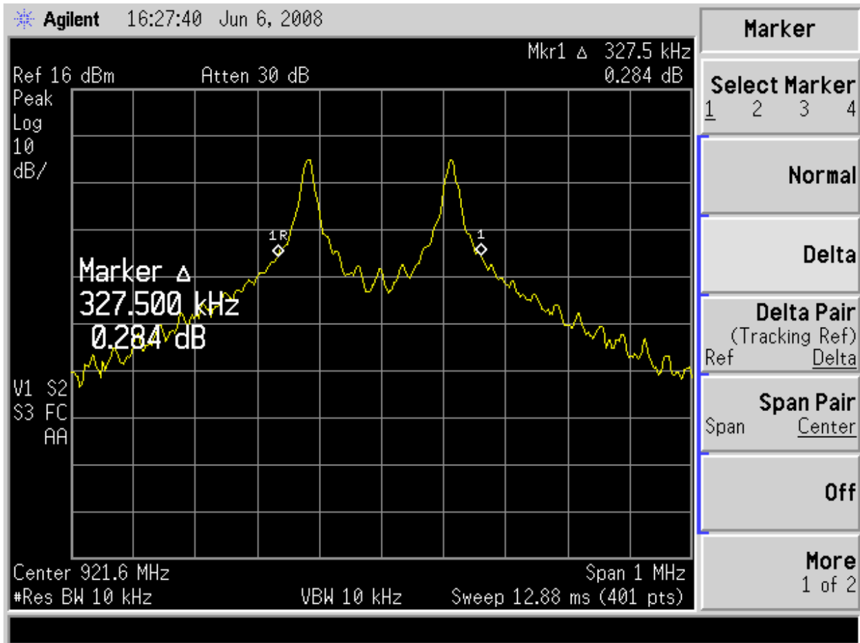
Figure 5 –921.6 MHz
