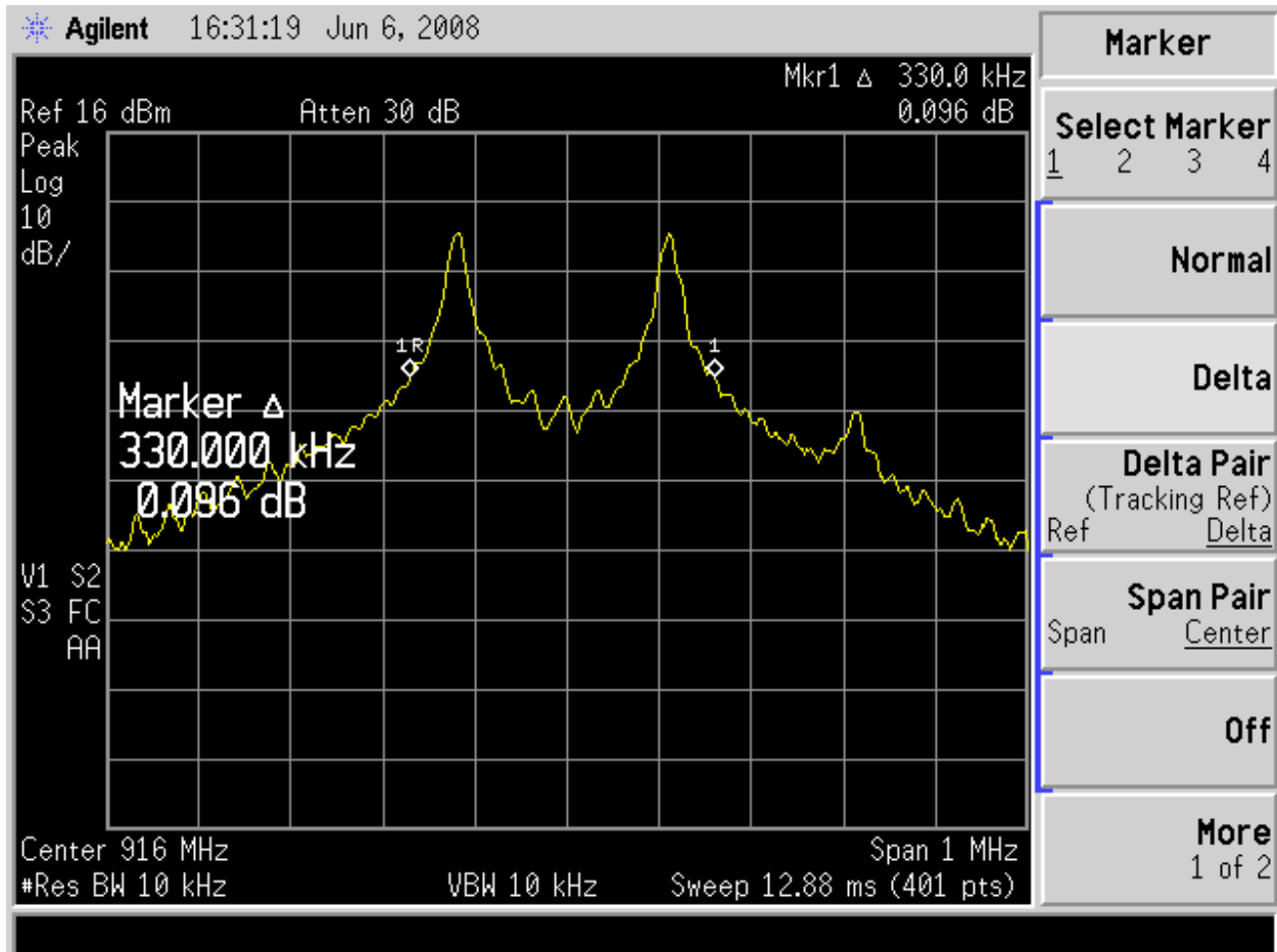
Figure 5 –916.0 MHz
