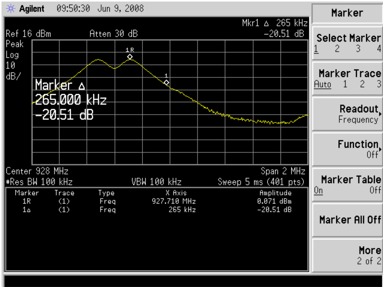
Figure 9 -927.6 MHz
