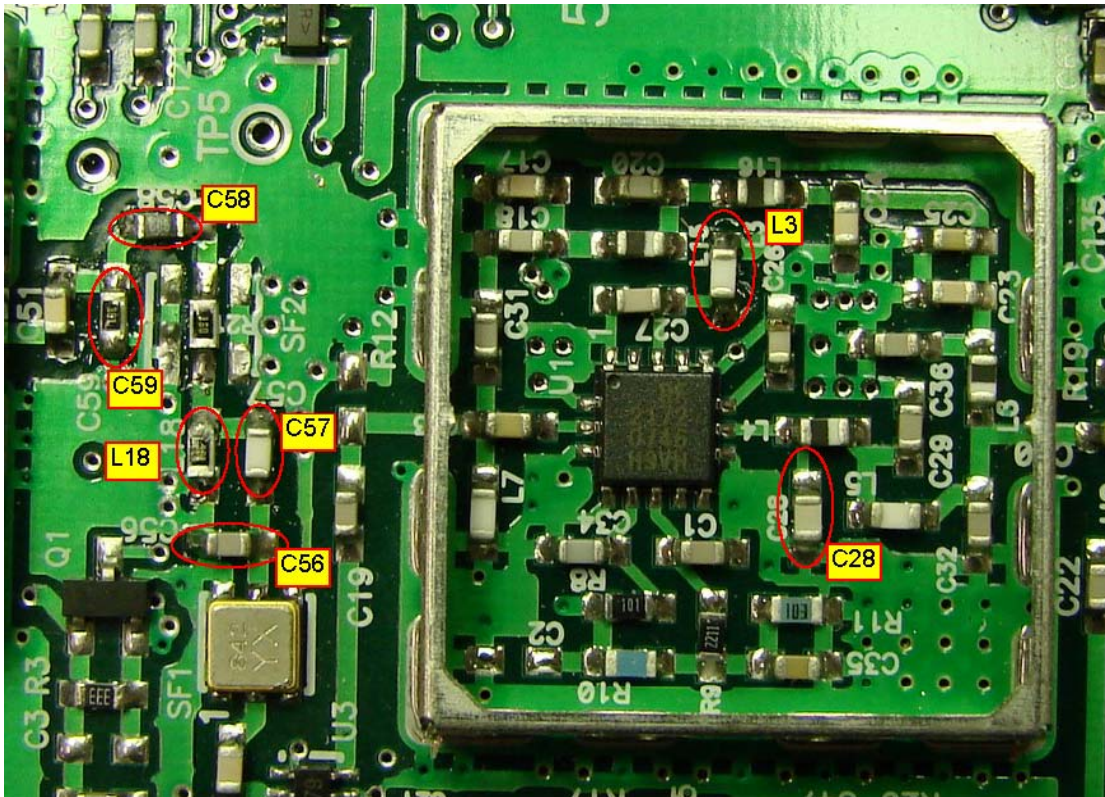
Changes to ILC2I PA shield cover is removed for clarity
