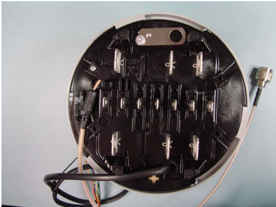
Host A3 Meter Exterior Rear View - Form 9S Shown
