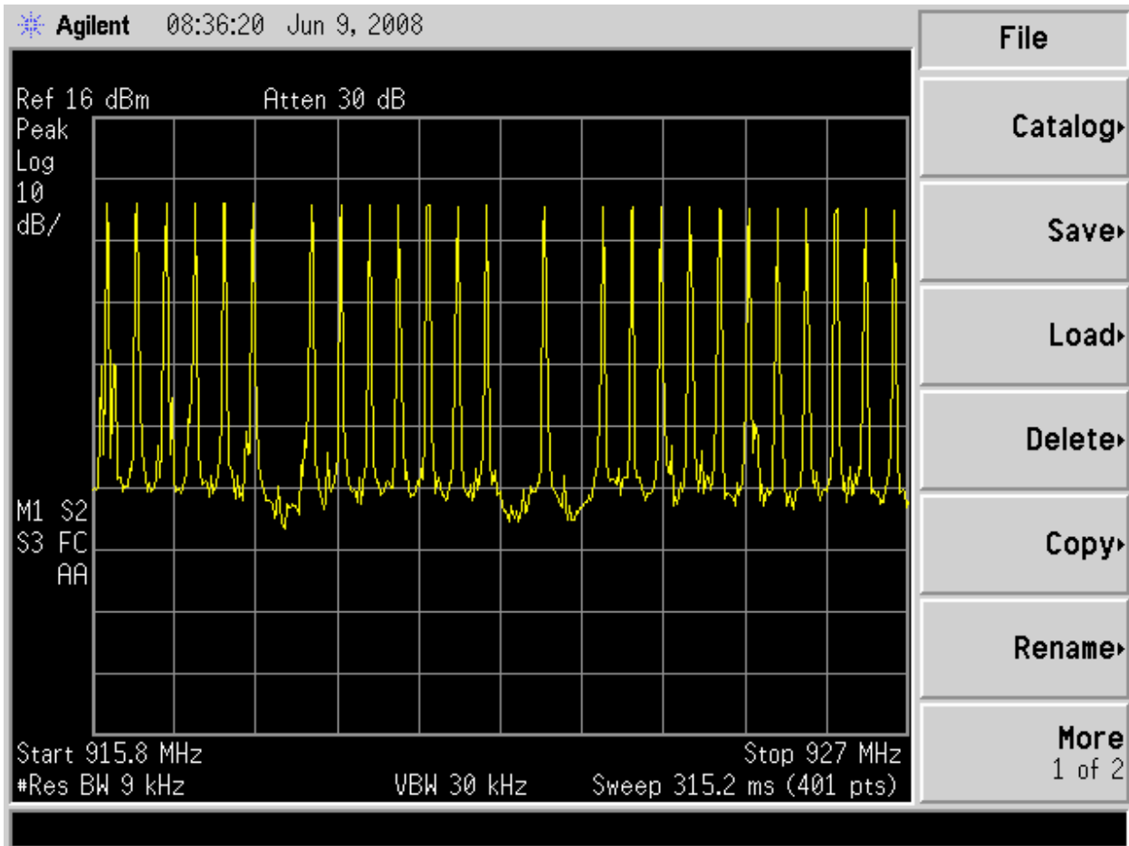
Figure 3 - Plot of available High Band Hopping Channels
