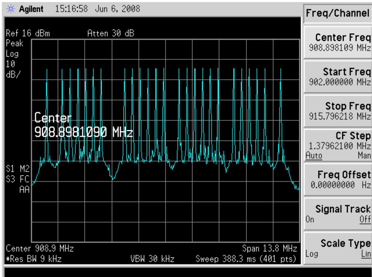
Figure 2 - Plot of available Low Band Hopping Channels
