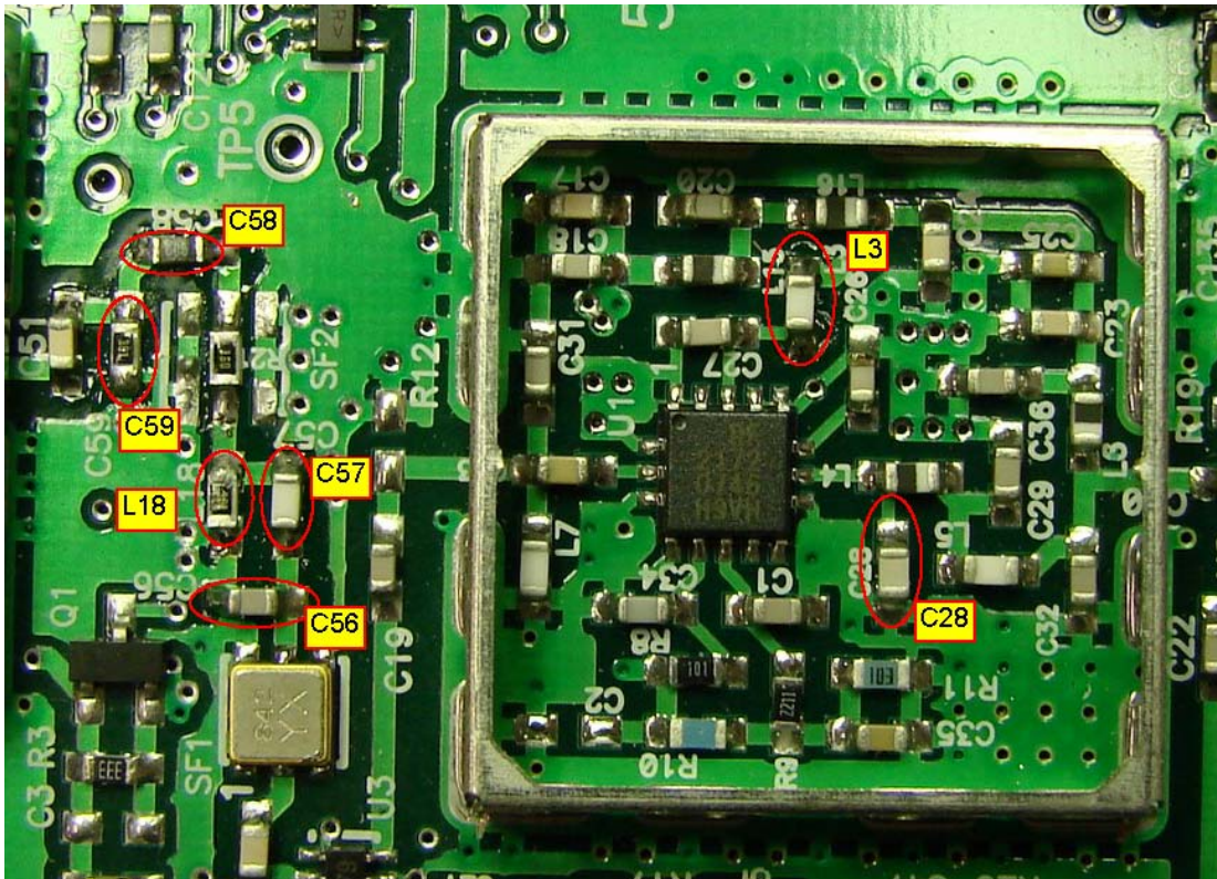
Changes to ILC2 PA shield cover is removed for clarity
