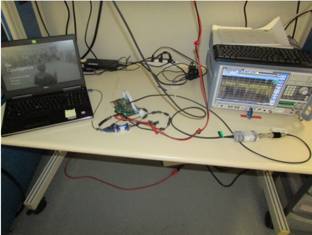
Figure 7: Conducted Emissions
