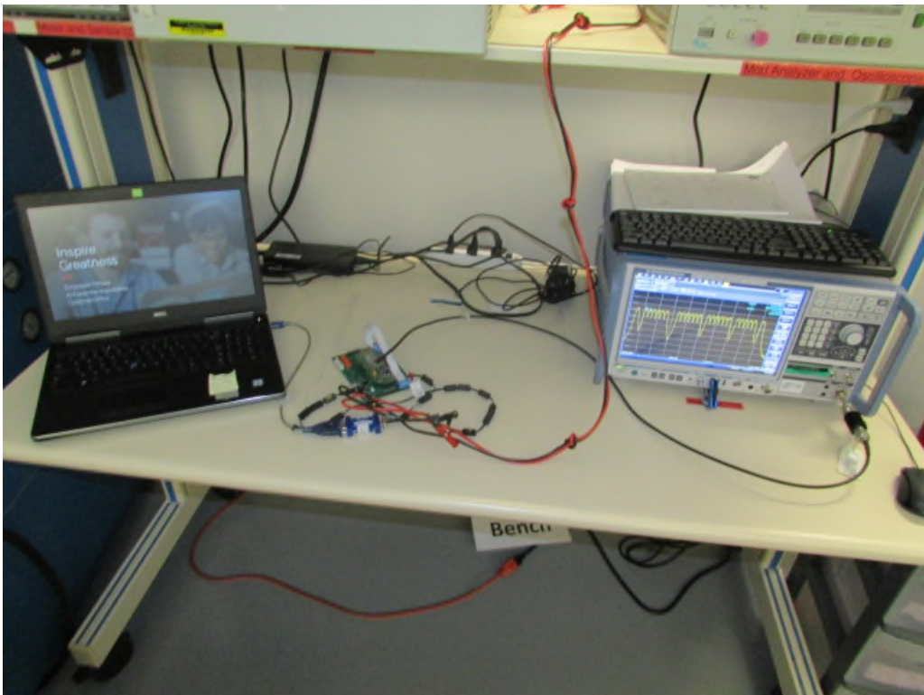
Figure 8: Conducted Emissions
