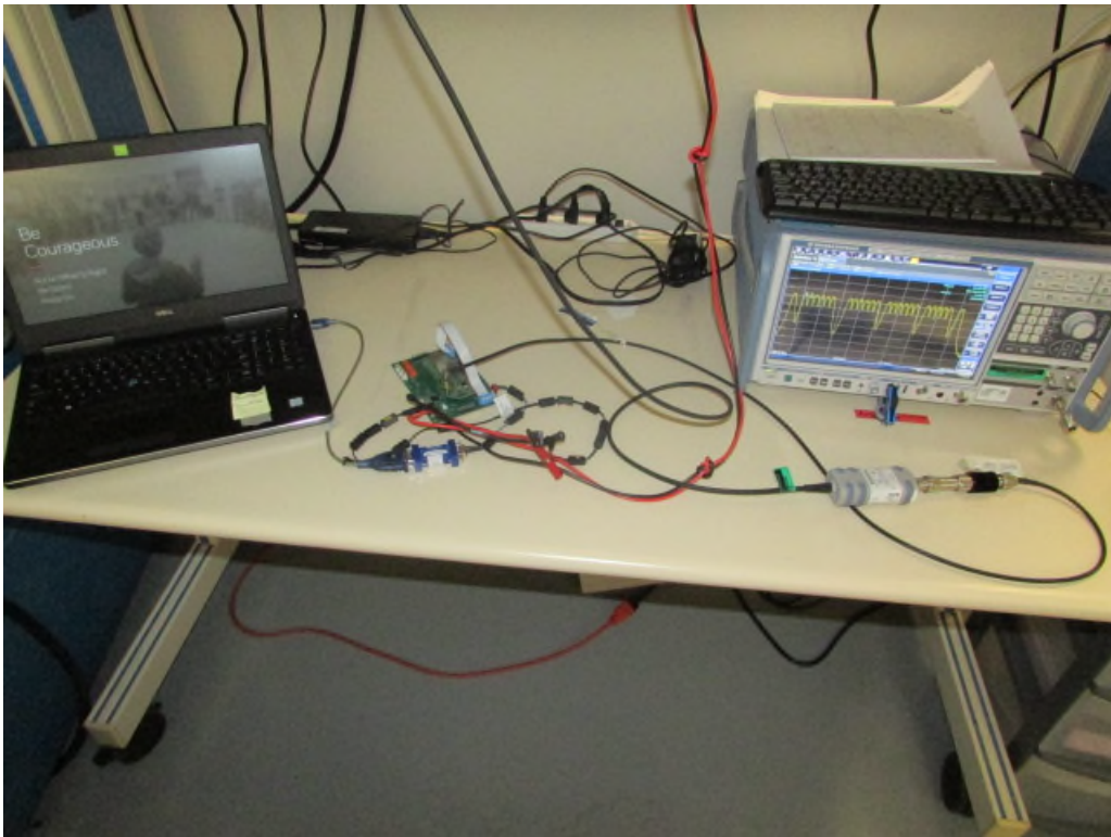
Figure 7: Conducted Emissions
