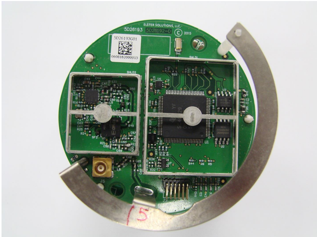
Radio PCBA, Top View, No Shields
