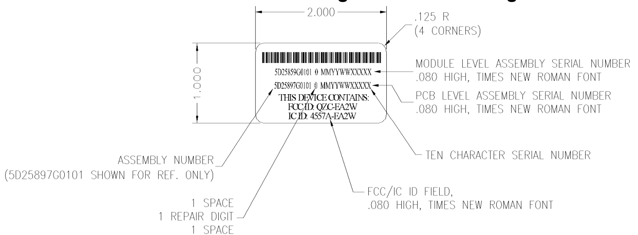
Figure 2: External FCC / IC Label drawing – Remote Housing
