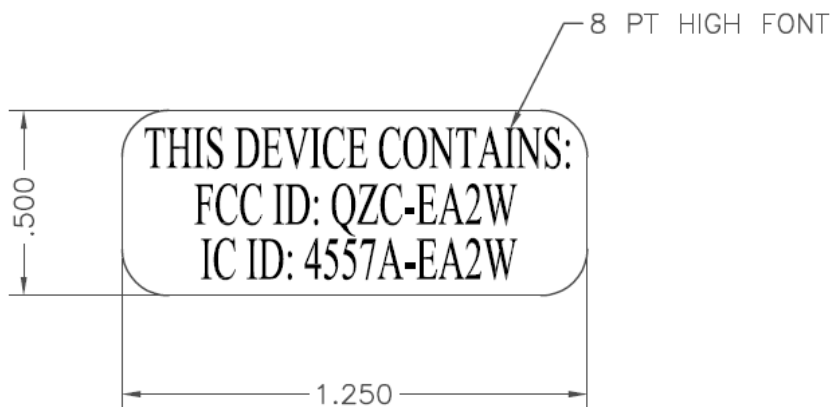
Figure 4: External FCC / IC Label drawing – Pit Housing
