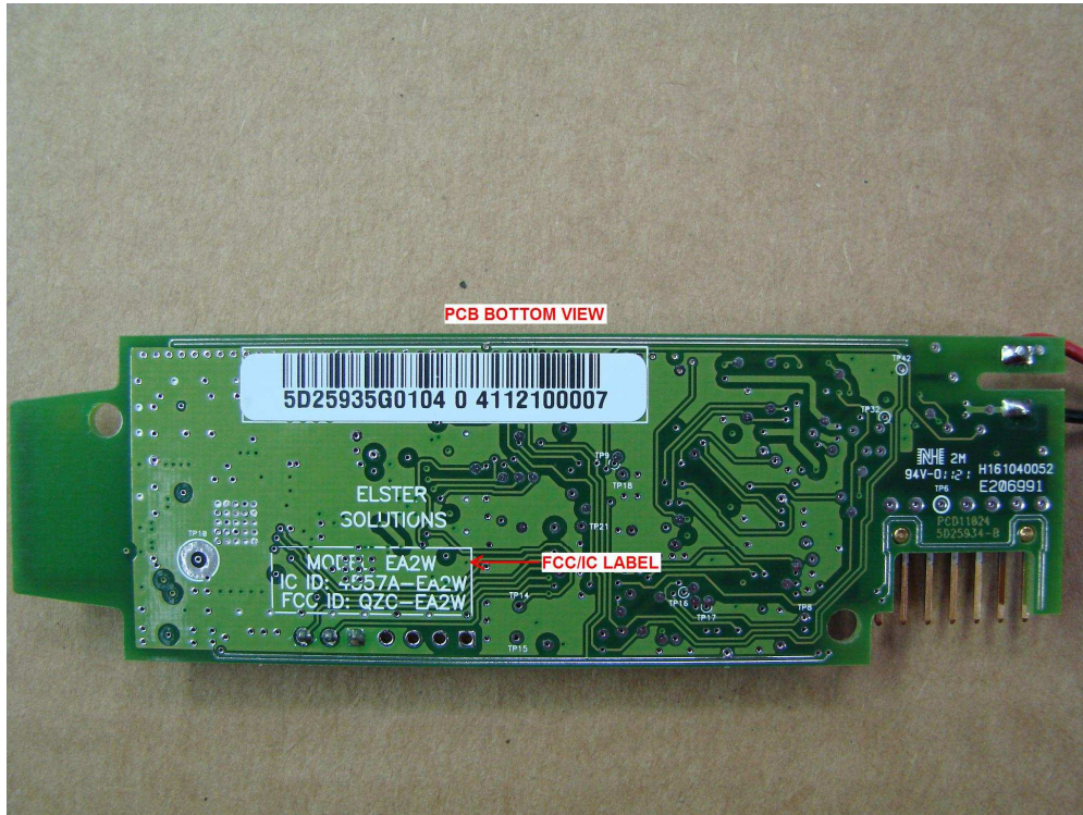
Figure 5: Location of Internal FCC / IC Label on EA2W Printed Circuit Board Assembly
