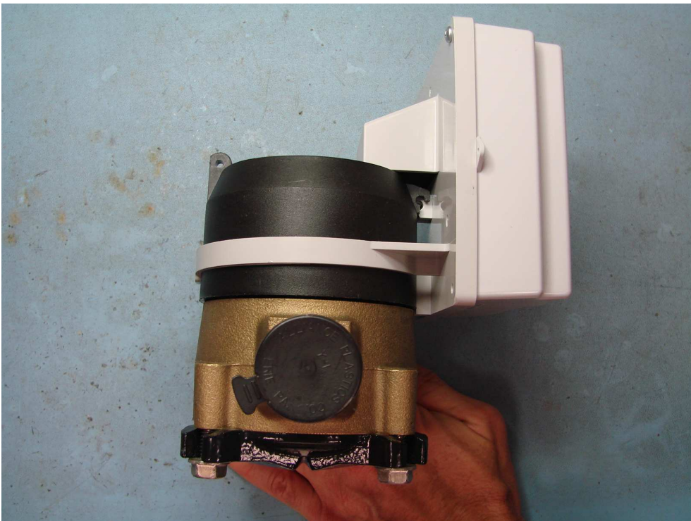
Figure 18: EA2W Integral Mount Module Left View
