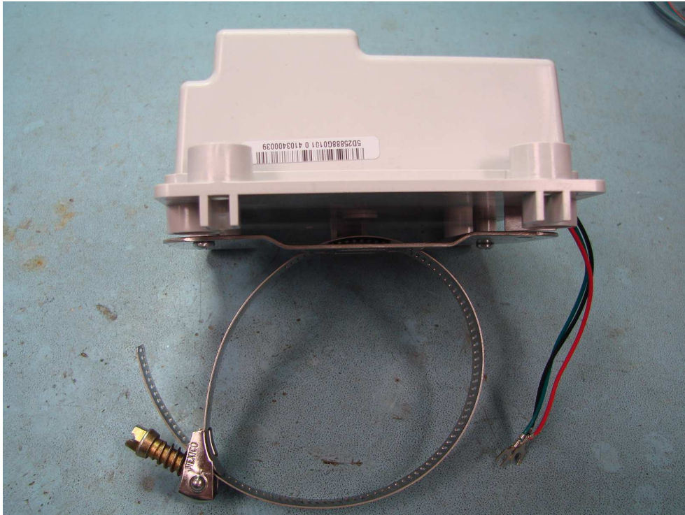
Figure 13: EA2W Pipe Mount Module Bottom View
