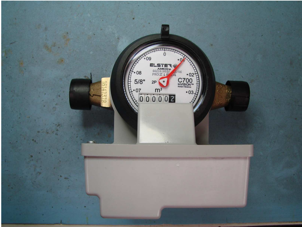
Figure 19: EA2W Integral Mount Module Top View
