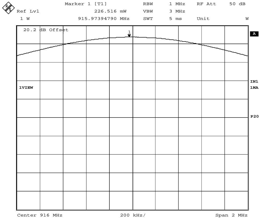
Figure 8: CH 34 (916.0 MHz) Peak Output Power - Worst Case Shown.
