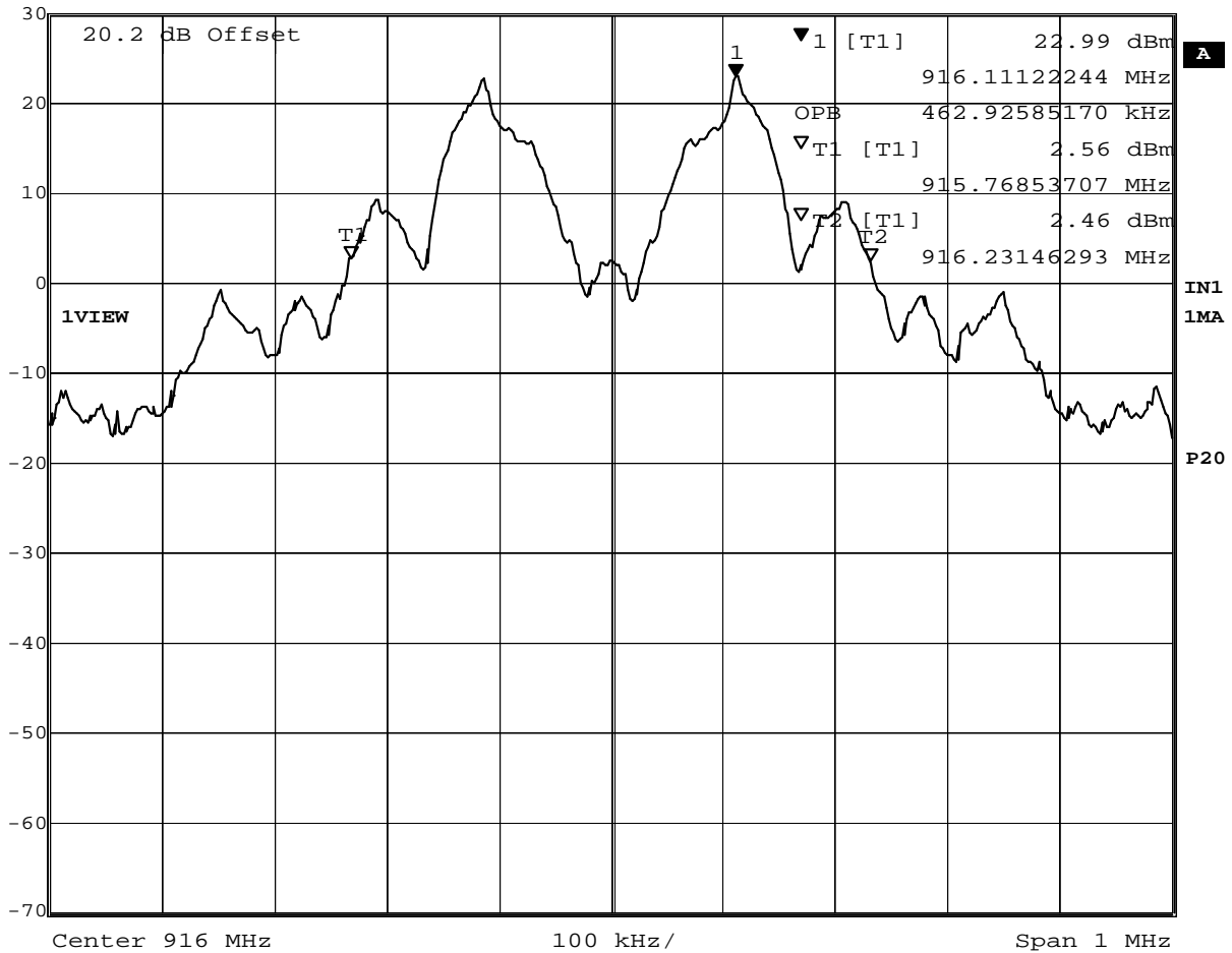
Figure 5 – 99% Power Bandwidth = 463 kHz
