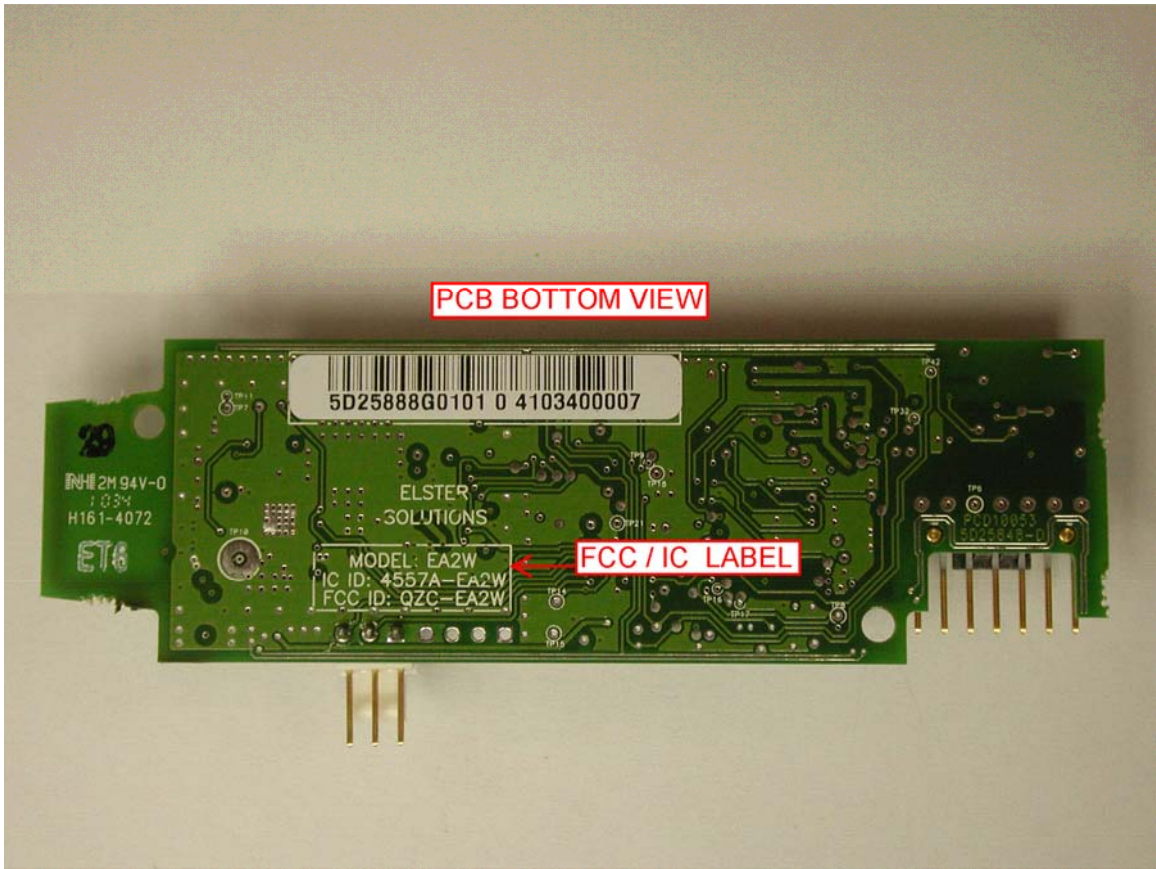
Figure 3: Location of Internal FCC / IC Label on EA2W Printed Circuit Board Assembly
