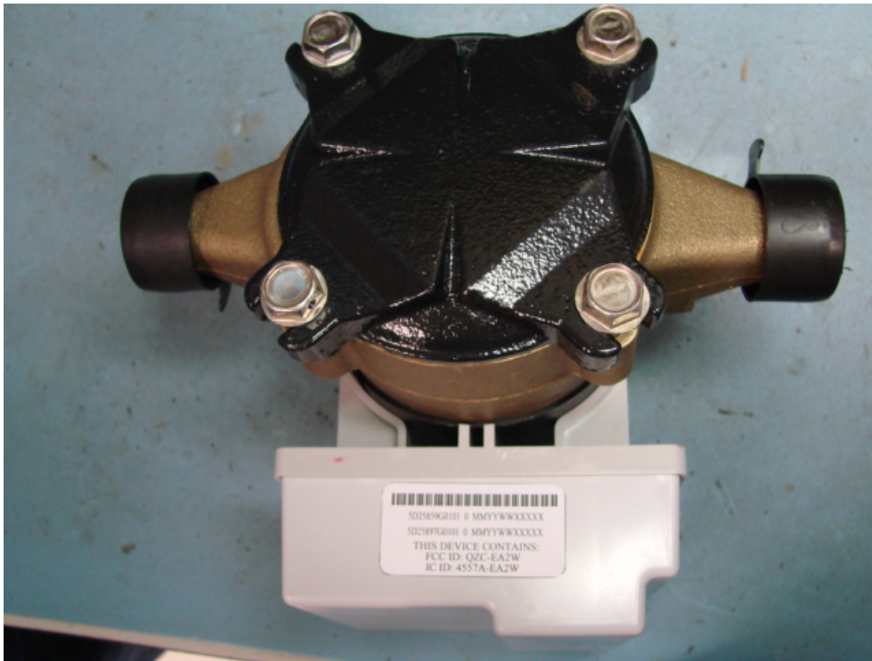
Figure 1: Location of External FCC / IC label on EA2W module
