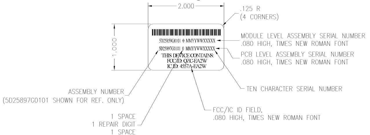
Figure 2: External FCC / IC Label drawing
