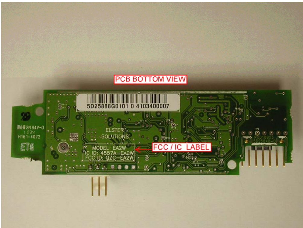
Figure 2: PCB Assembly Bottom View
