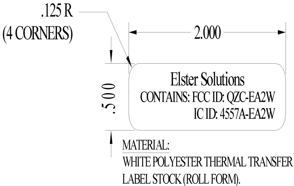
Figure 2: External FCC / IC Label drawing
