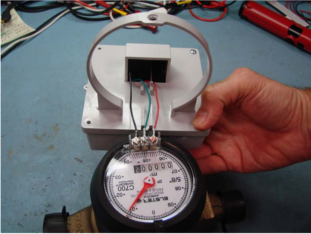
Figure 22: EA2W Integral Mount Module Assembly View 2
