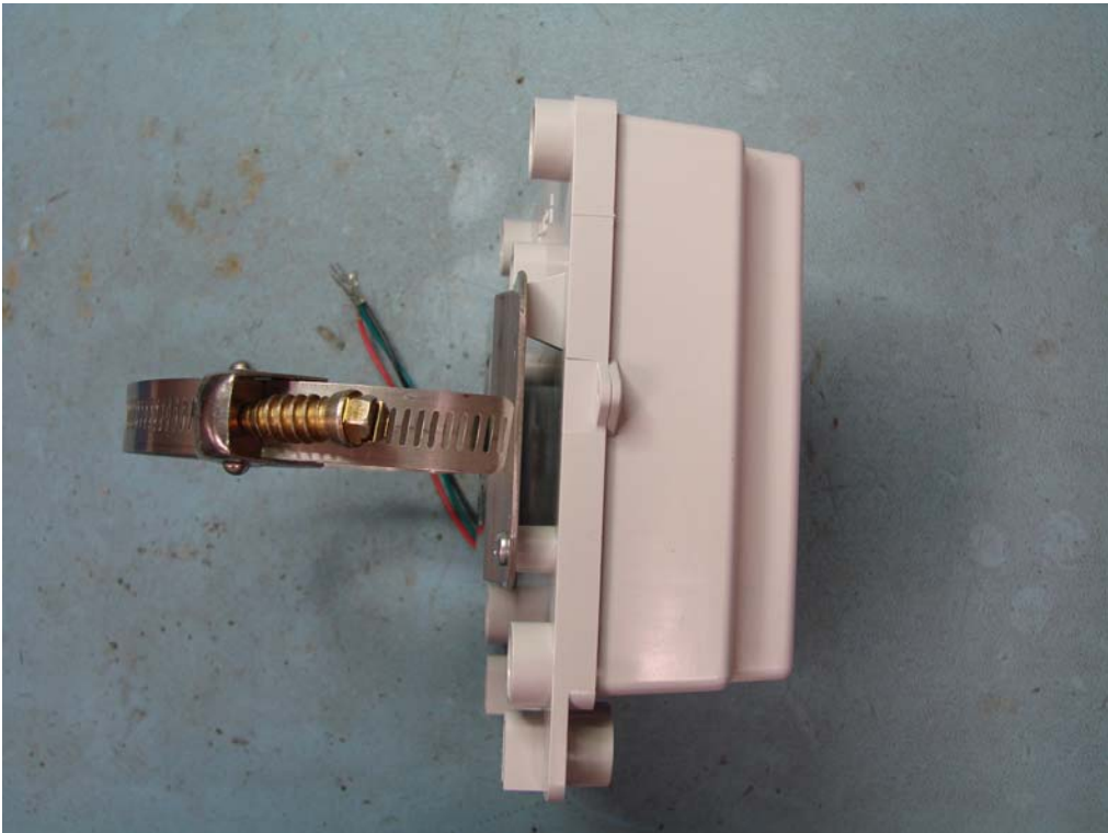
Figure 10: EA2W Pipe Mount Module Left View
