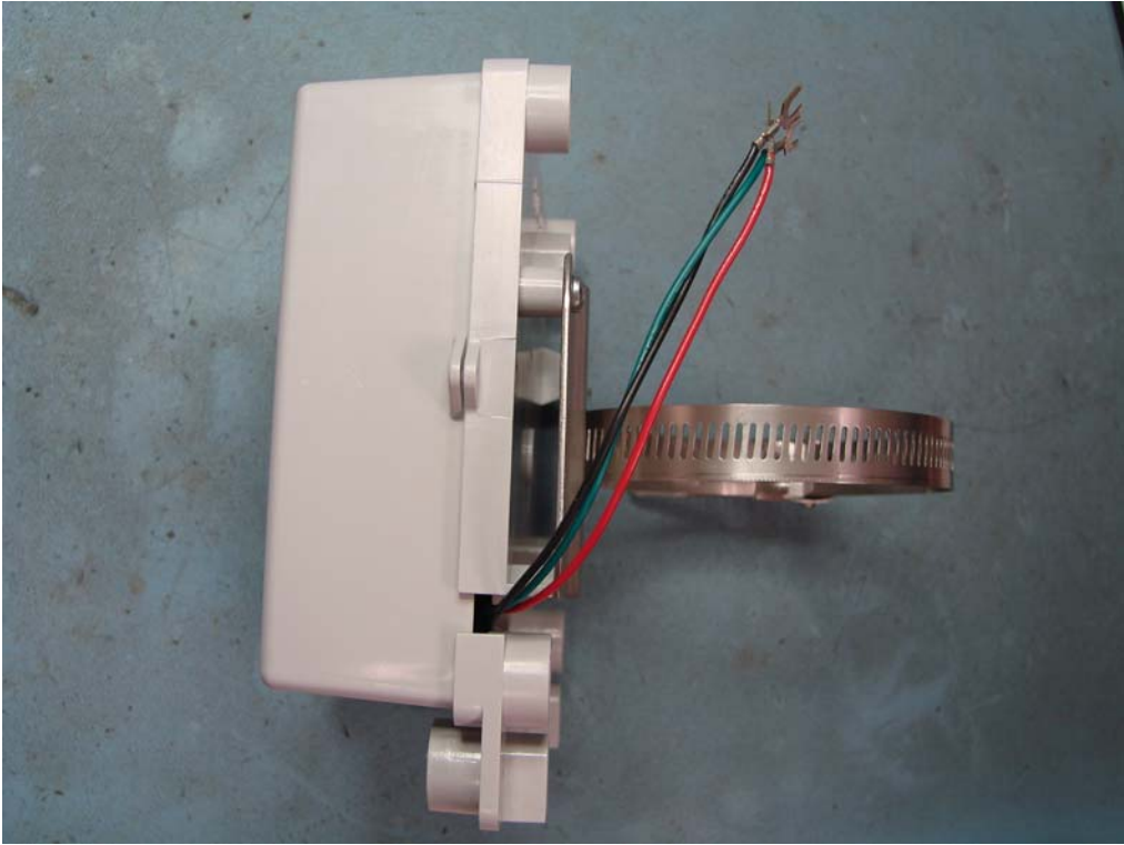
Figure 11: EA2W Pipe Mount Module Right View
