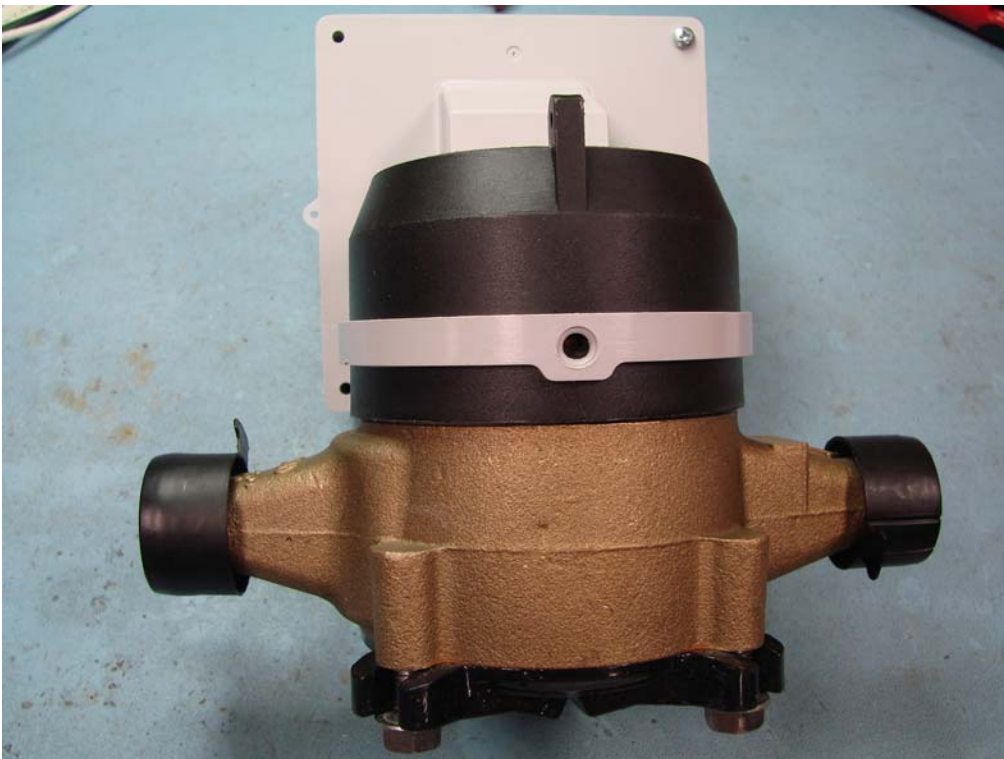
Figure 16: EA2W Integral Mount Module Rear View
