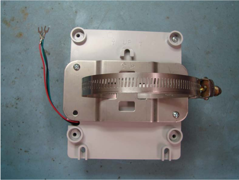
Figure 9: EA2W Pipe Mount Module Rear View
