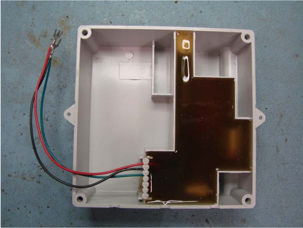
Figure 21: EA2W Integral Mount Module Assembly View 1
