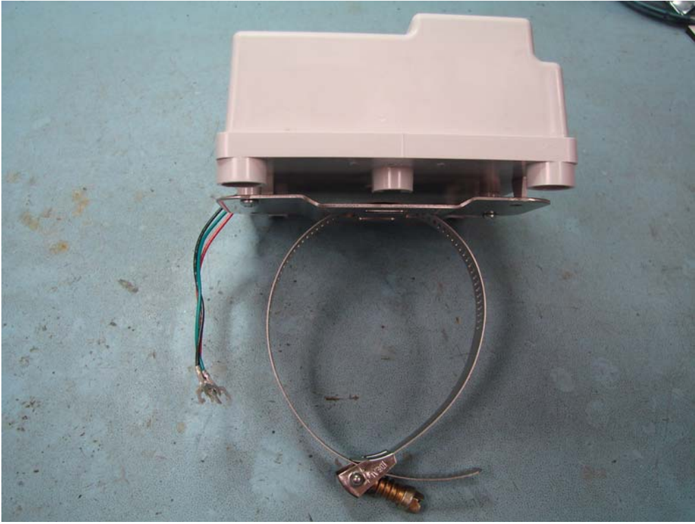
Figure 12: EA2W Pipe Mount Module Top View
