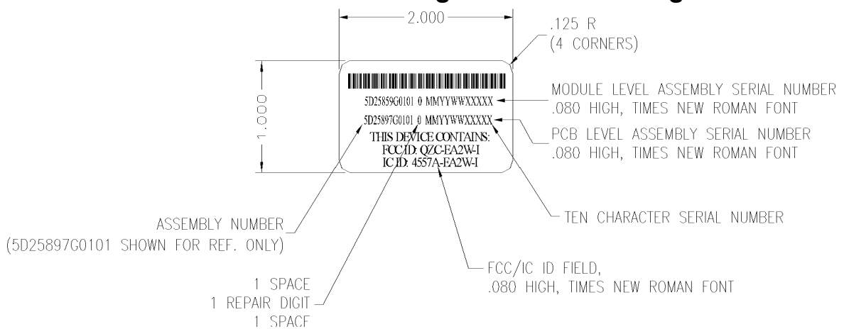
Figure 2: External FCC Label drawing – Remote Housing
