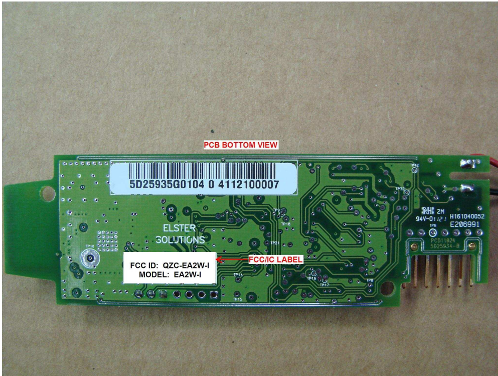
Figure 5: Location of Internal FCC Label on EA2W-I Printed Circuit Board Assembly (Bottom)
