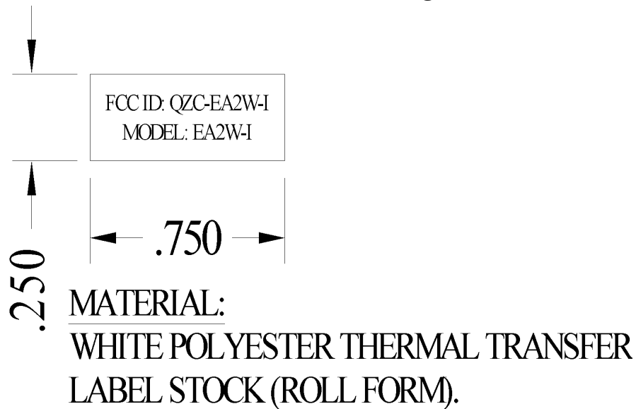
Figure 6: Internal FCC Label Drawing
