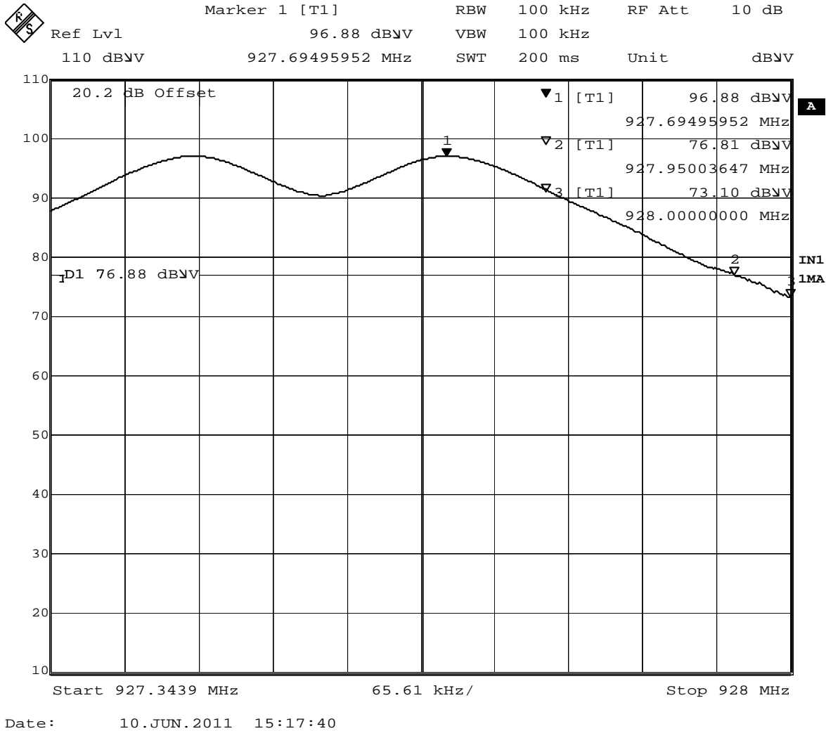
Figure 6: Upper Band Edge Measurement
