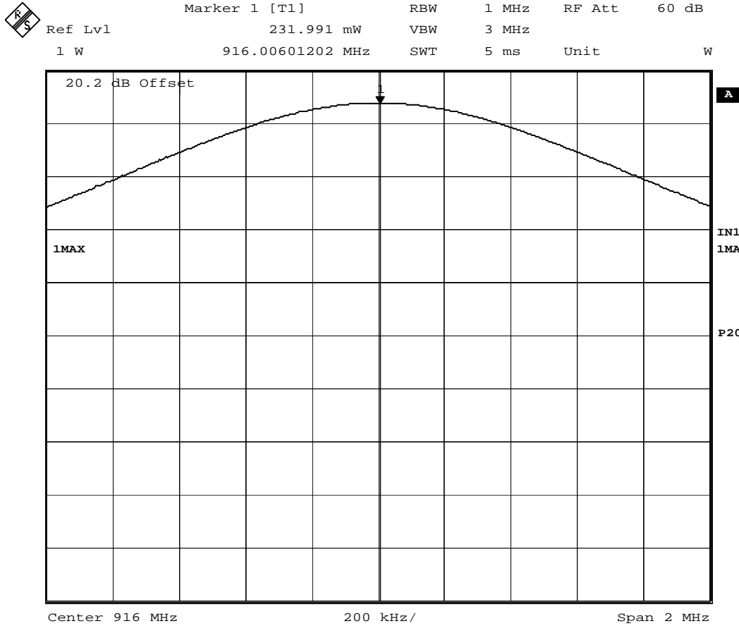
Figure 7: CH 34 (916.0 MHz) Peak Output Power - Worst Case Shown.
