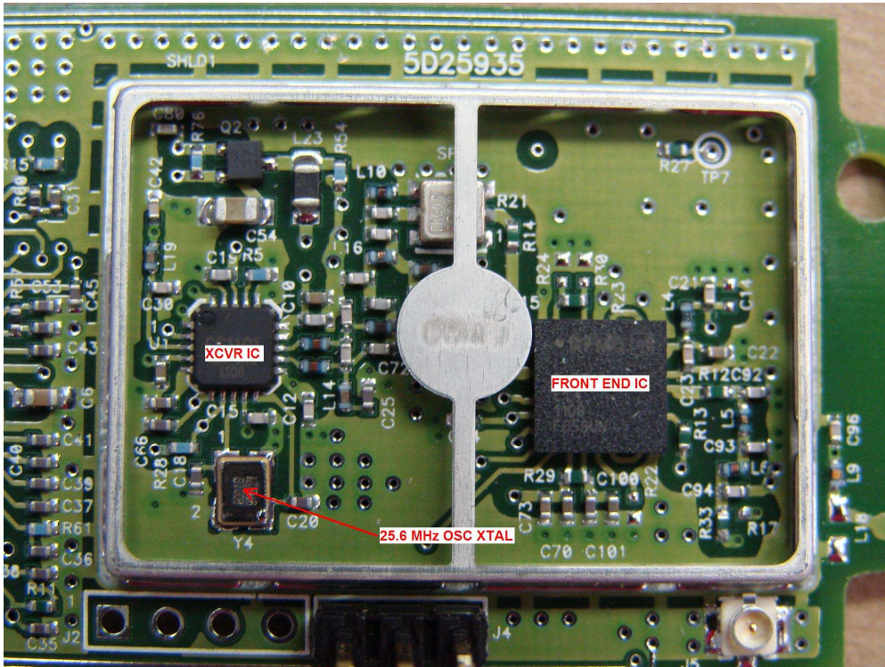
Figure 3: Transceiver Circuitry under Shield
