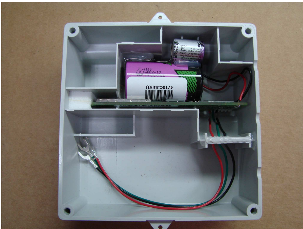
Figure 4: Assembled module prior to Potting
