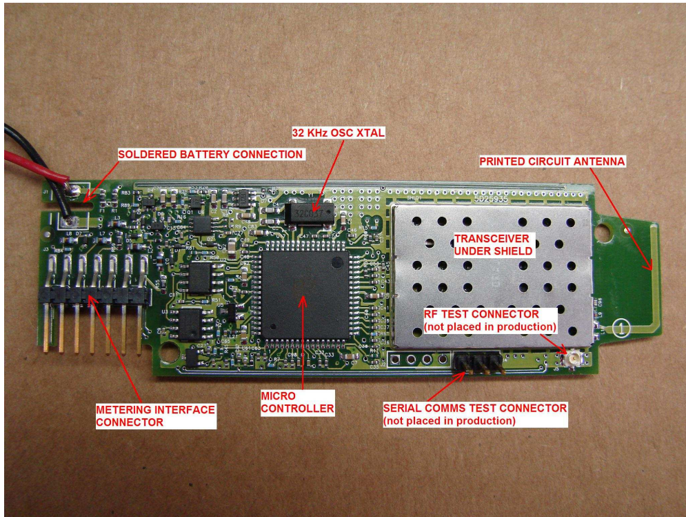
Figure 1: PCB Assembly Top View
