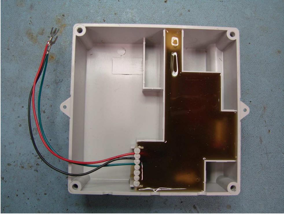
Figure 5: Assembled module after potting
