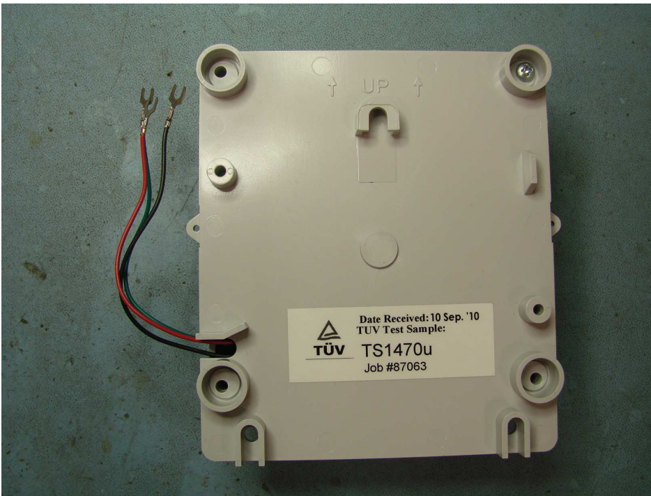
Figure 2: EA2W-I Remote Wall Mount Module Rear View
