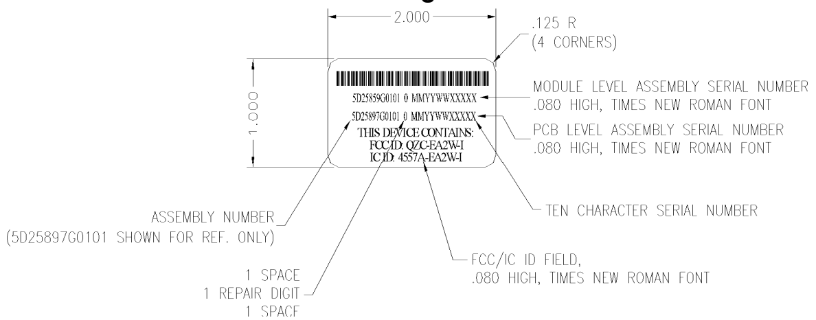
Figure 2: External FCC Label drawing
