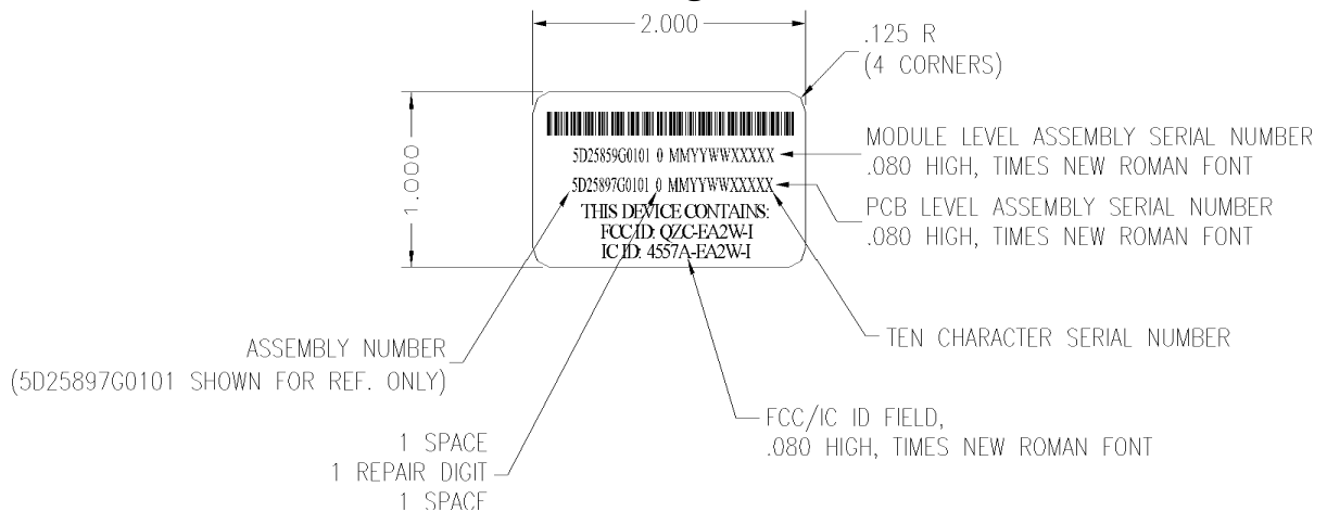
Figure 2: External FCC Label drawing
