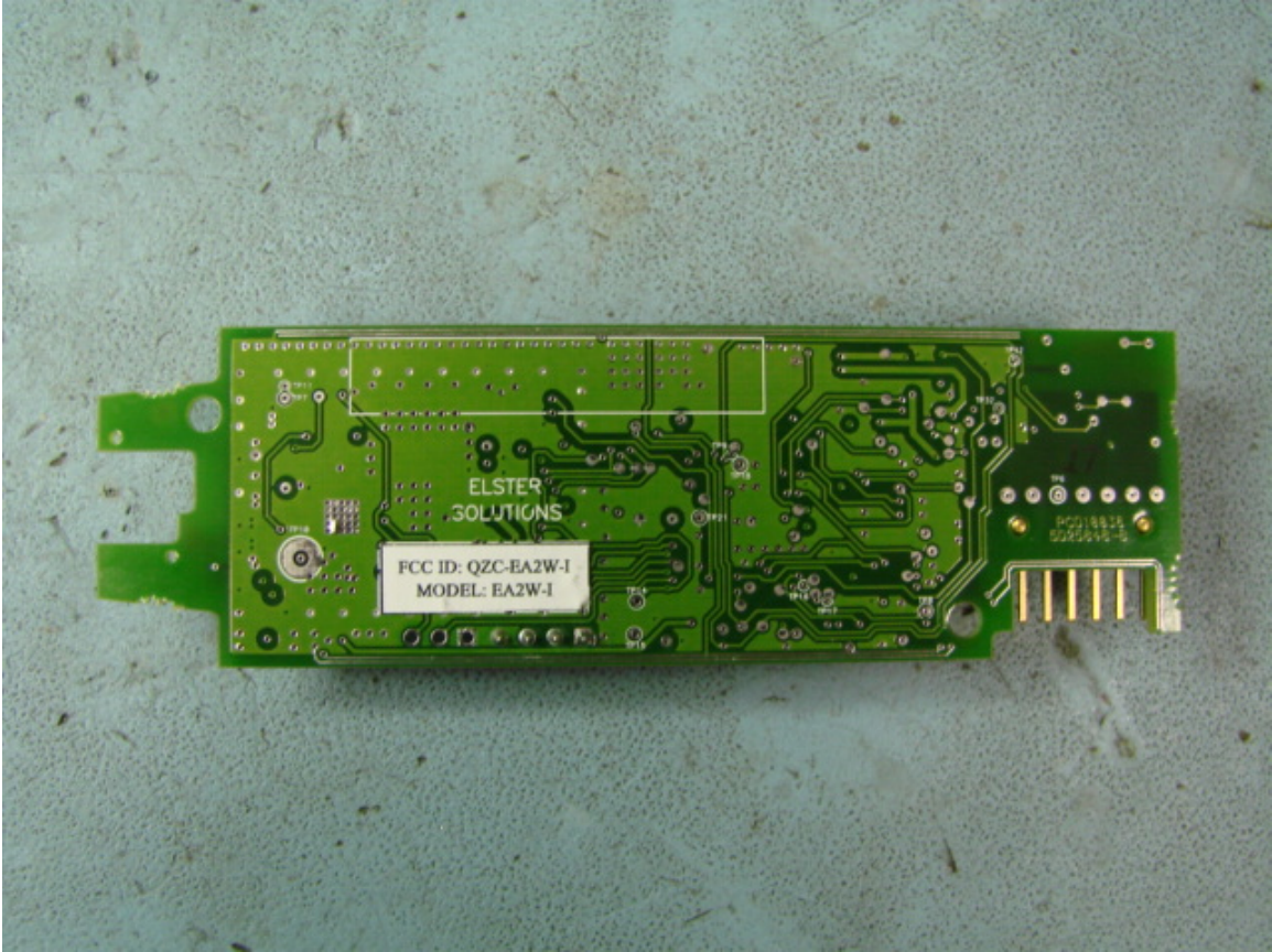
Figure 3: Location of Internal FCC Label on EA2W-I Printed Circuit Board Assembly (Bottom)
