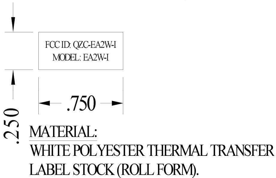
Figure 4: Internal FCC Label Drawing
