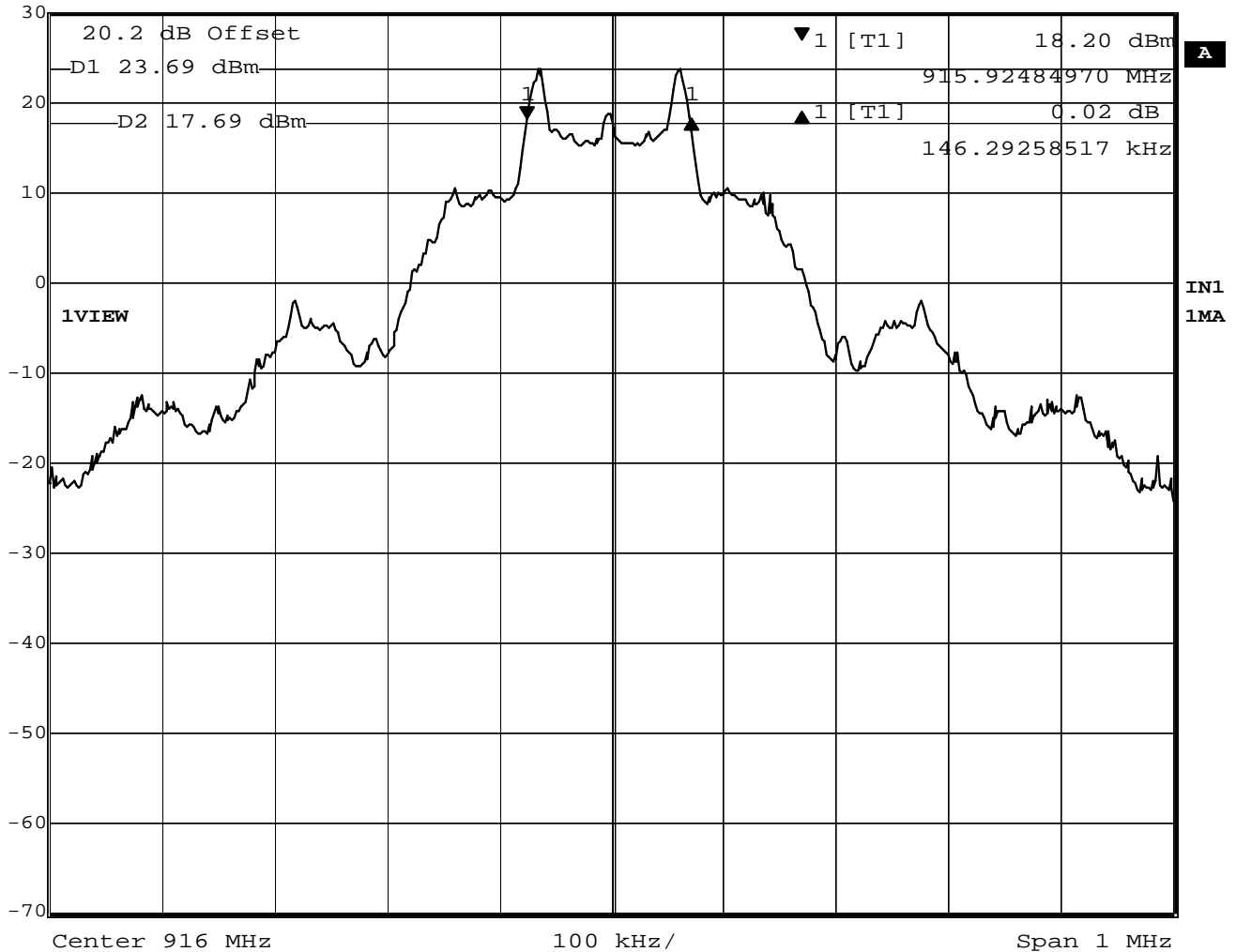
Figure 5: Occupied Bandwidth
