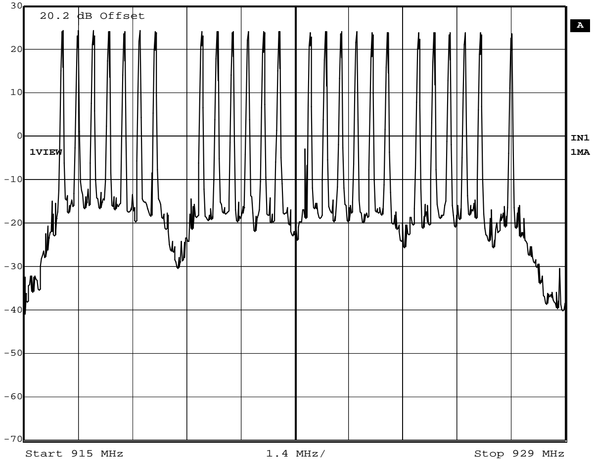
Figure 2: Plot of hopping Channels - 915-928 MHz
