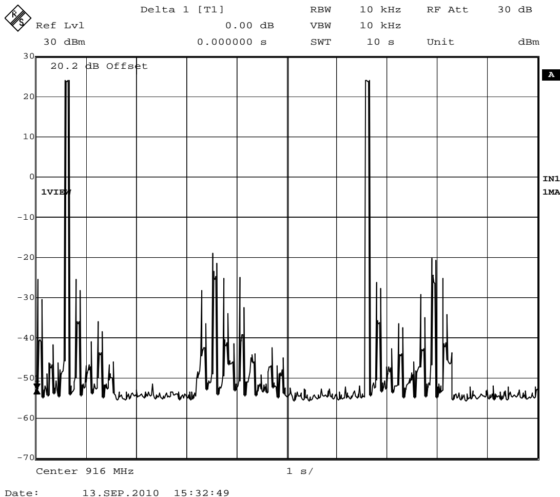
Figure 3: 10 second sweep of 916 MHz
