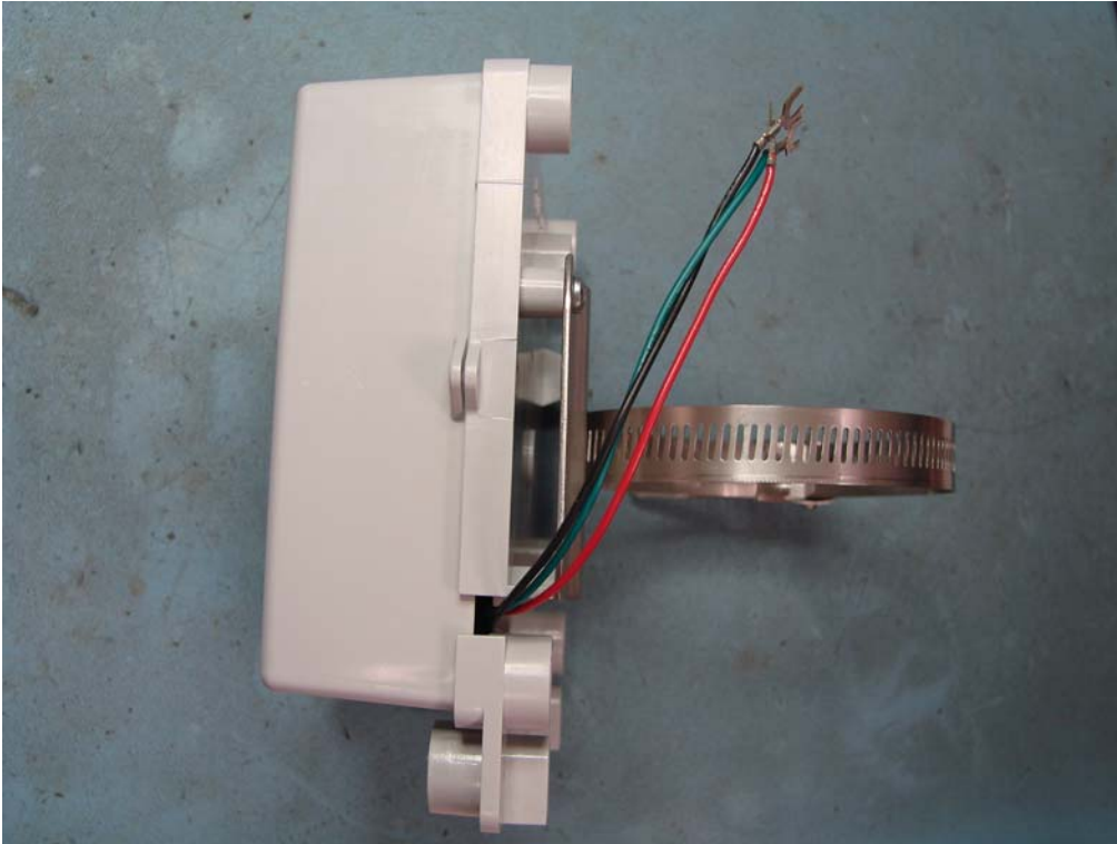
Figure 11: EA2W-I Pipe Mount Module Right View
