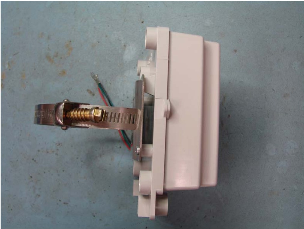
Figure 10: EA2W-I Pipe Mount Module Left View
