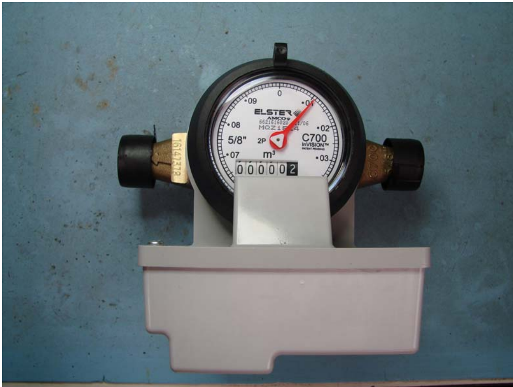
Figure 19: EA2W-I Integral Mount Module Top View
