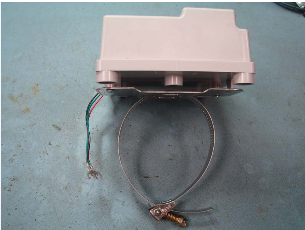
Figure 12: EA2W-I Pipe Mount Module Top View
