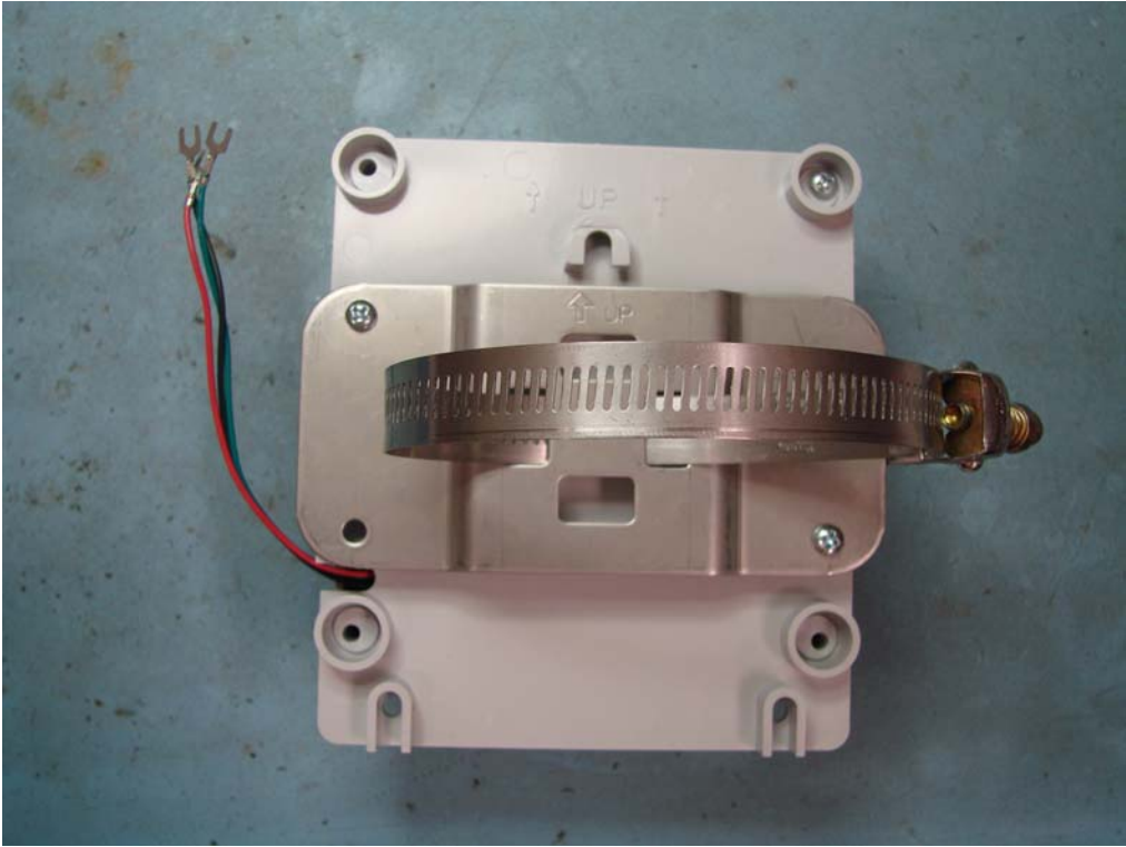
Figure 9: EA2W-I Pipe Mount Module Rear View
