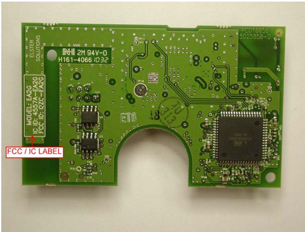
Location of Internal FCC / IC Label on EA2G Printed Circuit Board Assembly
