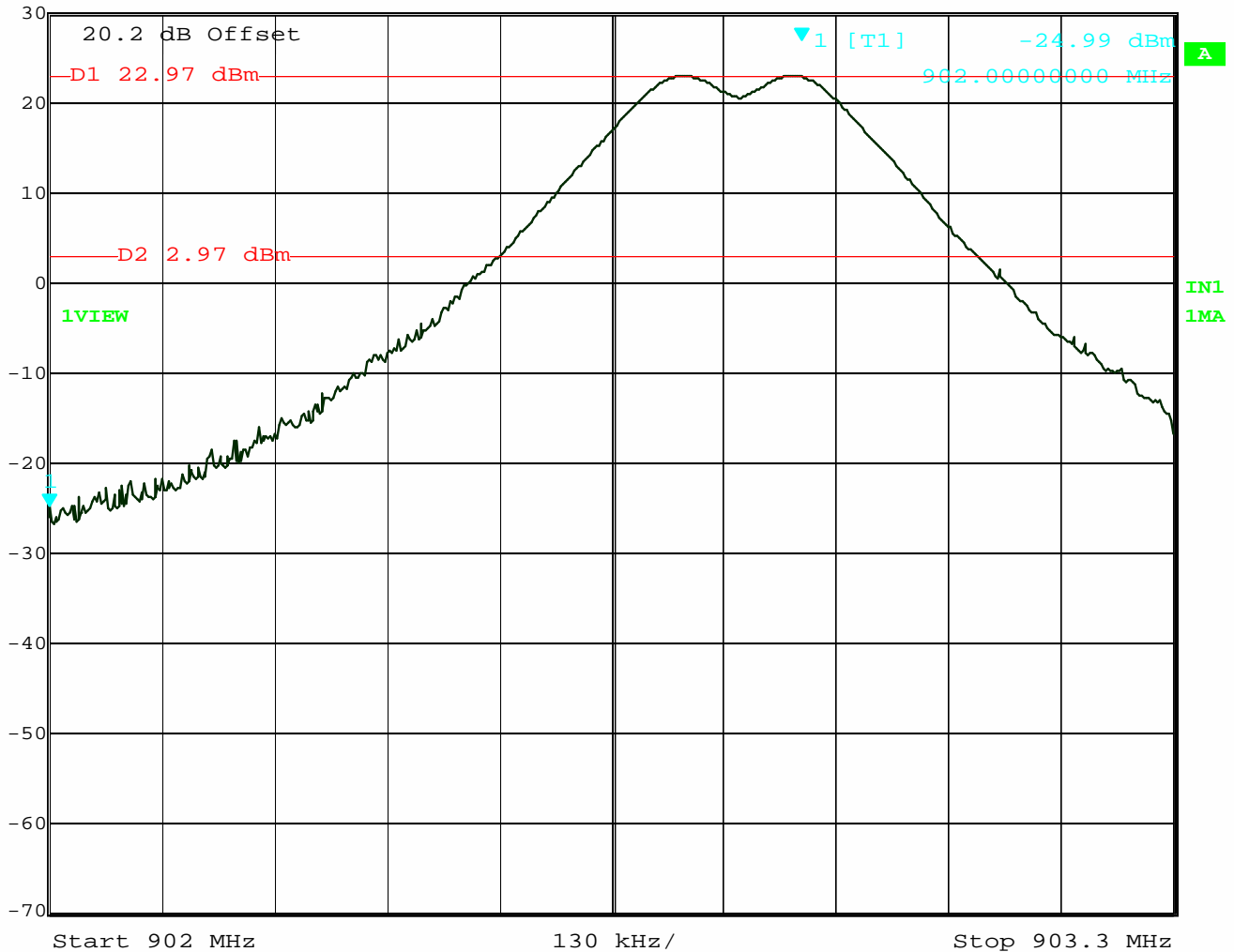
Figure 9: Lower Band Edge Measurement
