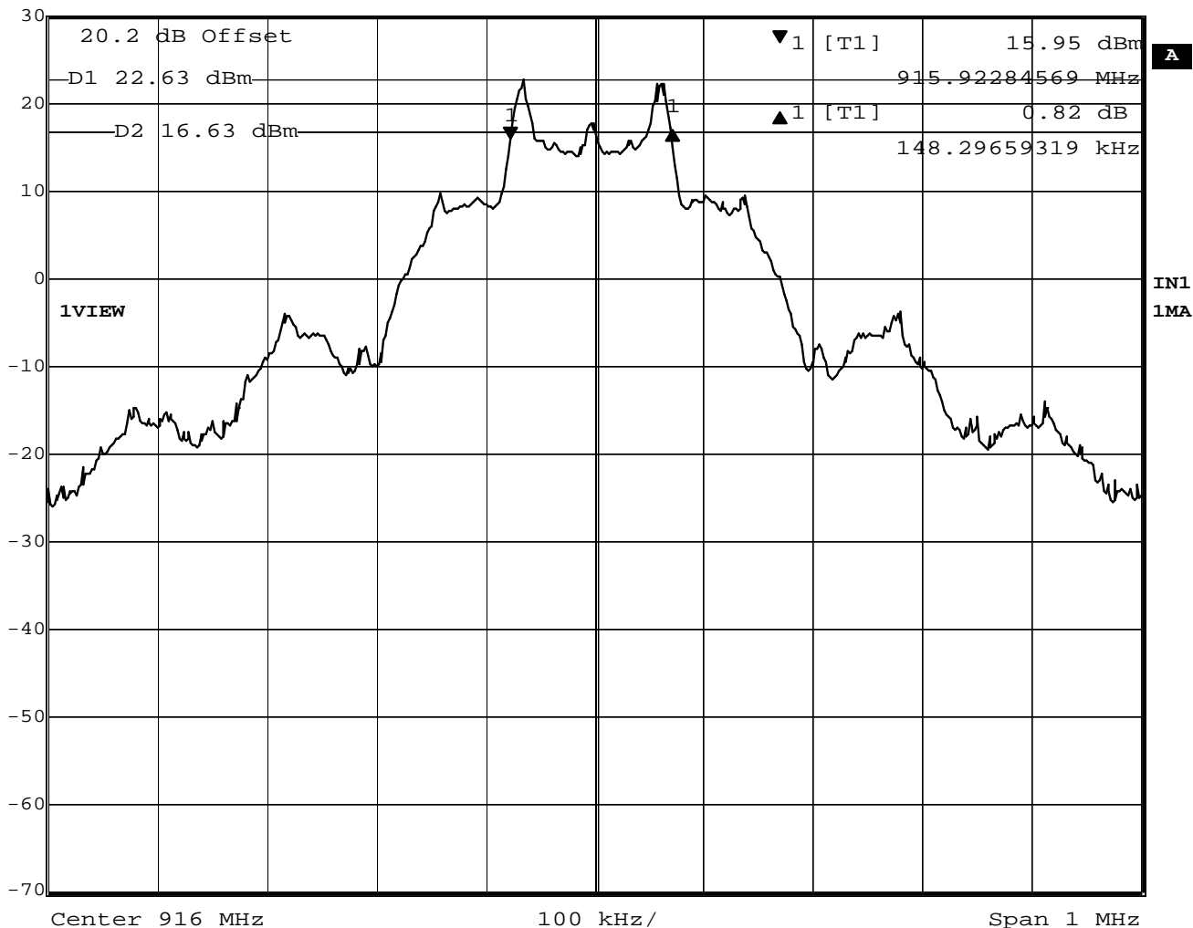
Figure 6: 6 dB Occupied Bandwidth
