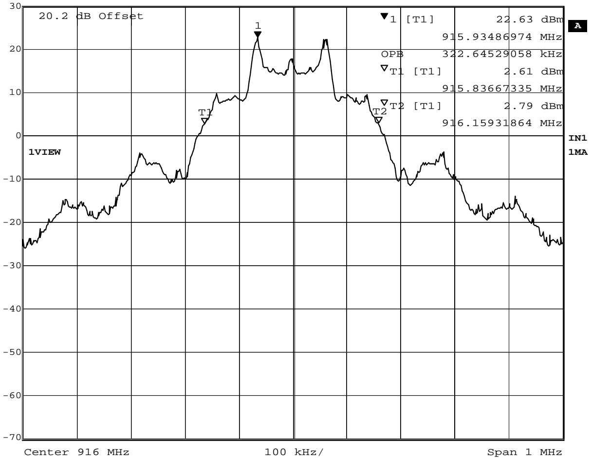
Figure 8 – 99% Power Bandwidth = 322.6 kHz
