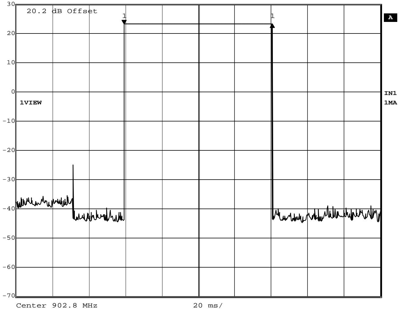
Figure 5: Measurement of 1 hop at 902.8 MHz
